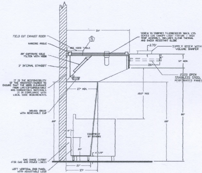
SECTION VIEW - MODEL 5412SND-2 HOOD - #1 (LEFT) WITH 266 MISC-PSP SUPPLY PLENUM
