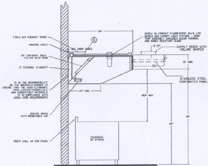
SECTION VIEW - MODEL 5412SND-2 HOOD - #2 (RIGHT) WITH 288 MISC-PSP SUPPLY PLENUM
