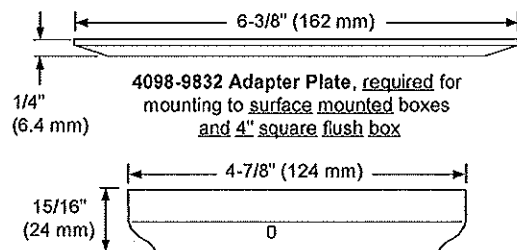
TrueAlarm Bases 4098-9789, -9791, & -9792
