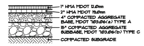
PAVEMENT SECTION NOT TO SCALE
