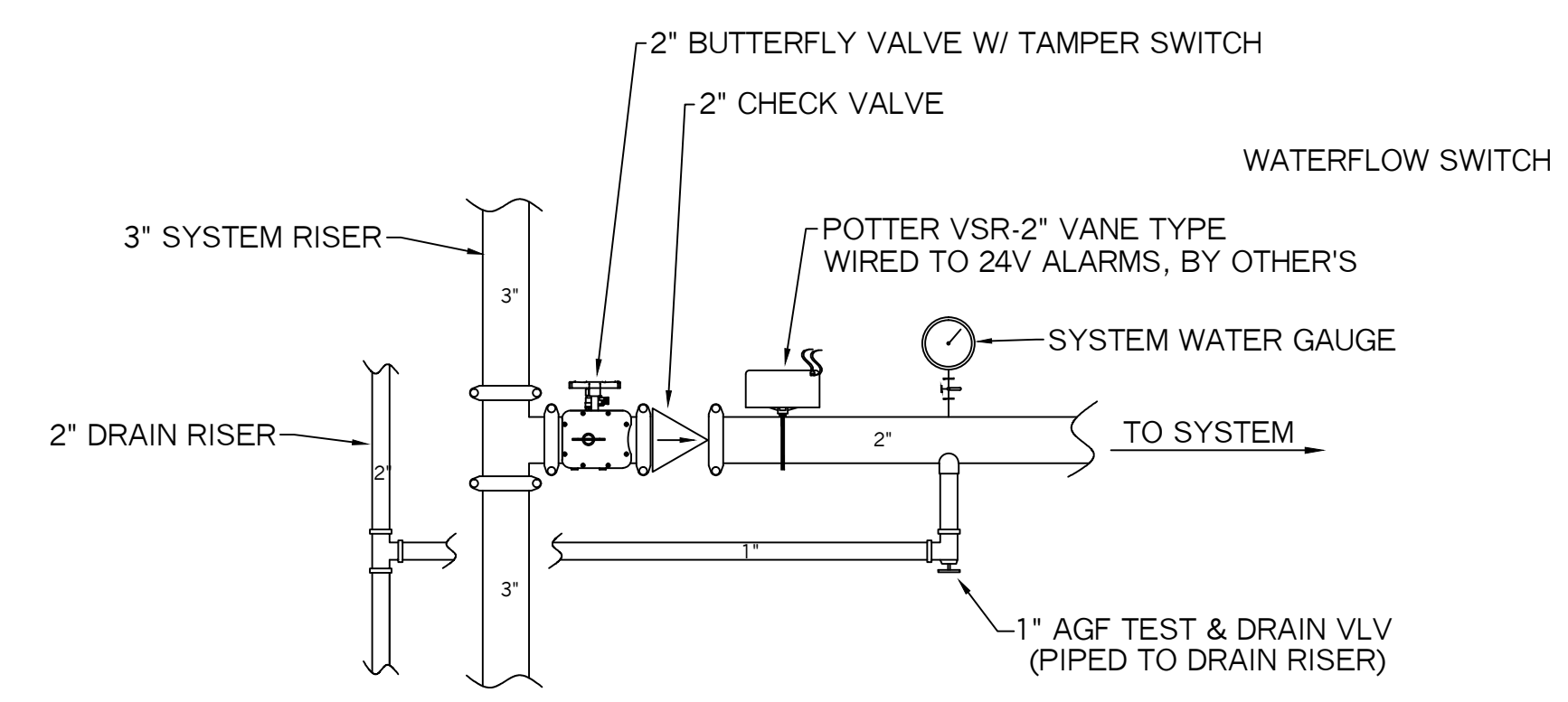
FLOOR CONTROL ASSEMBLY DETAIL N.T.S.
