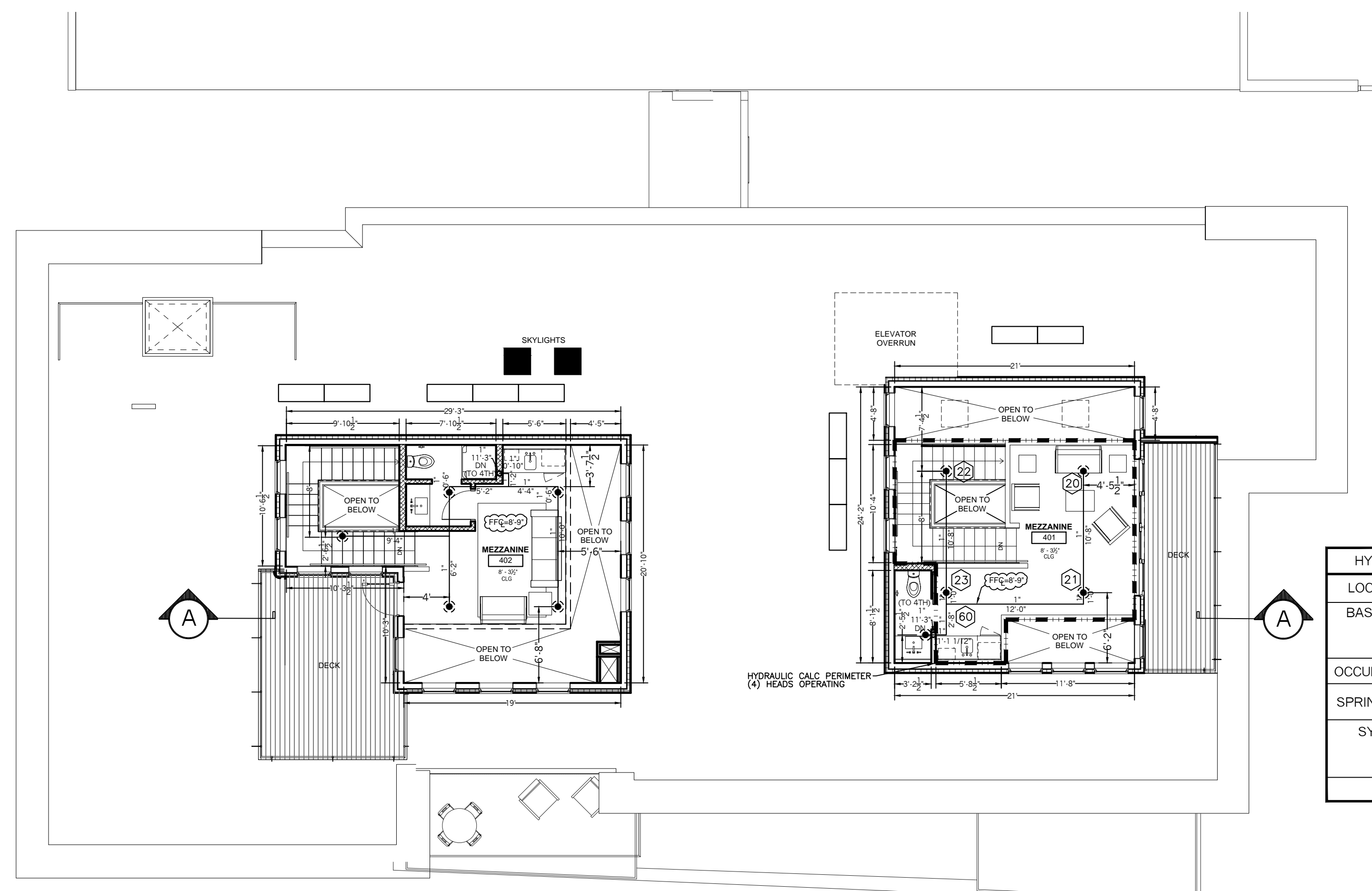
MEZZANINE FLOOR PLAN SCALE: 1/8" = 1'-0" FLOOR AREA = 880 SF FF ELEV. 72.83'
