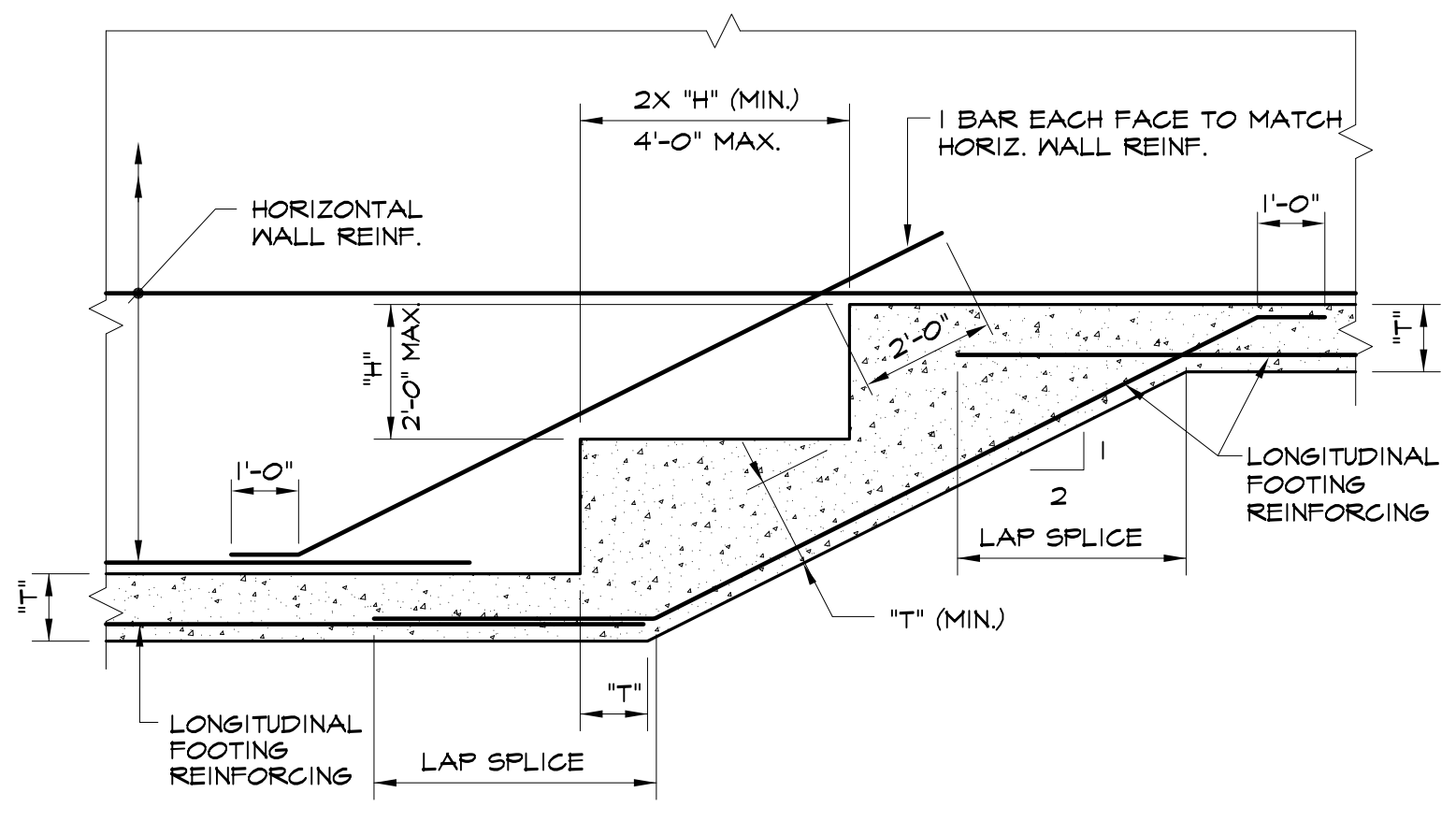
CONTINUOUS STEPPED WALL FOOTING
