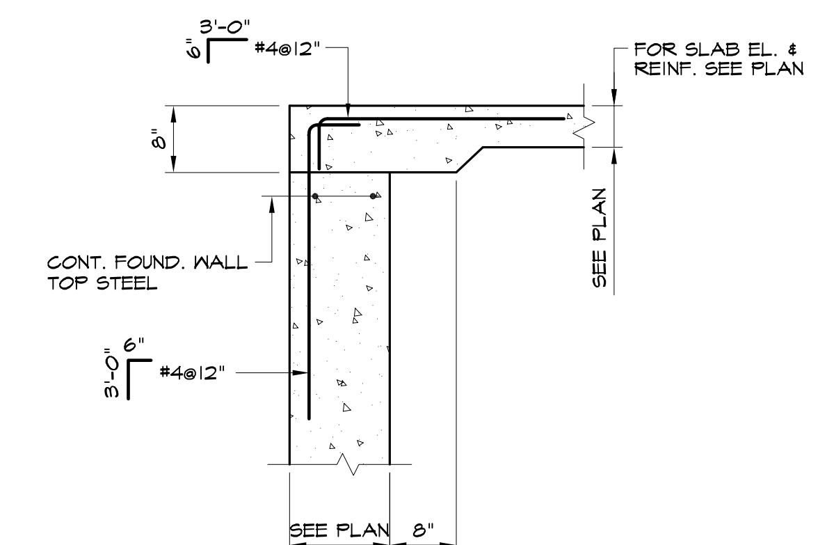
TYPICAL WALL SECTION AT DOORWAY TOW ELEVATION = -0'-8"
