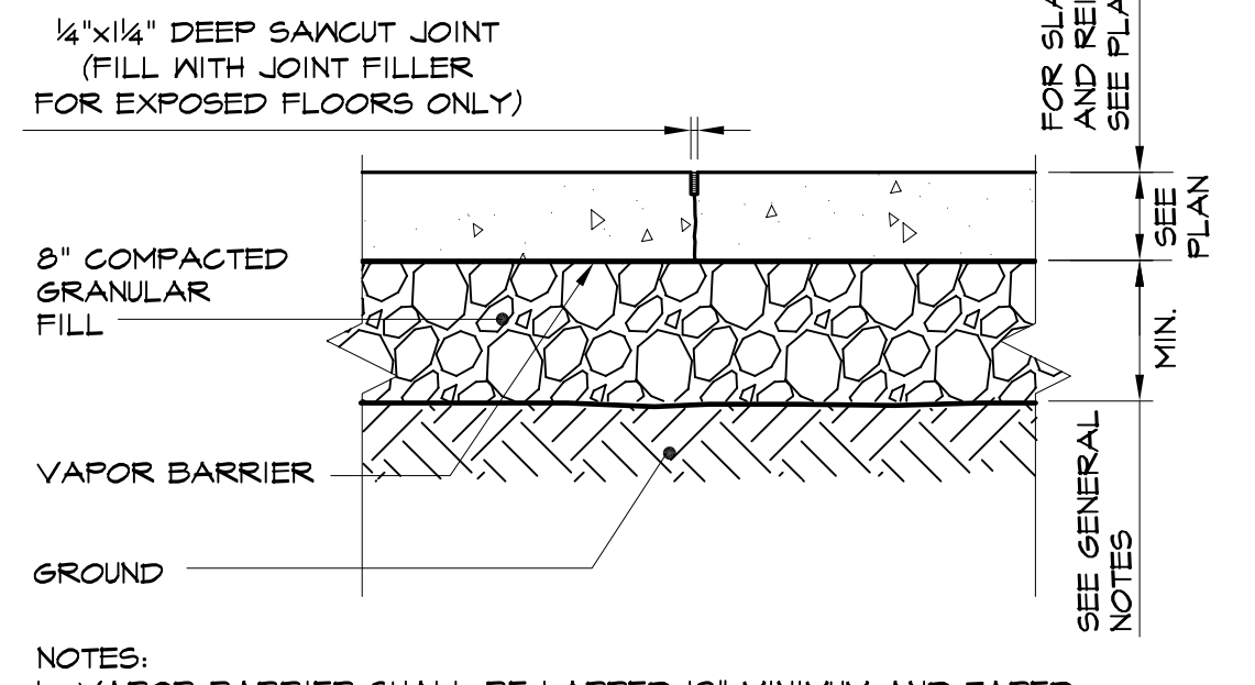
TYPICAL SAW CUT DETAIL CONTROL JOINT DETAIL
