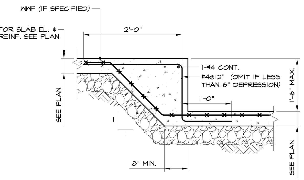
DEPRESSION AT SLAB ON GRADE
