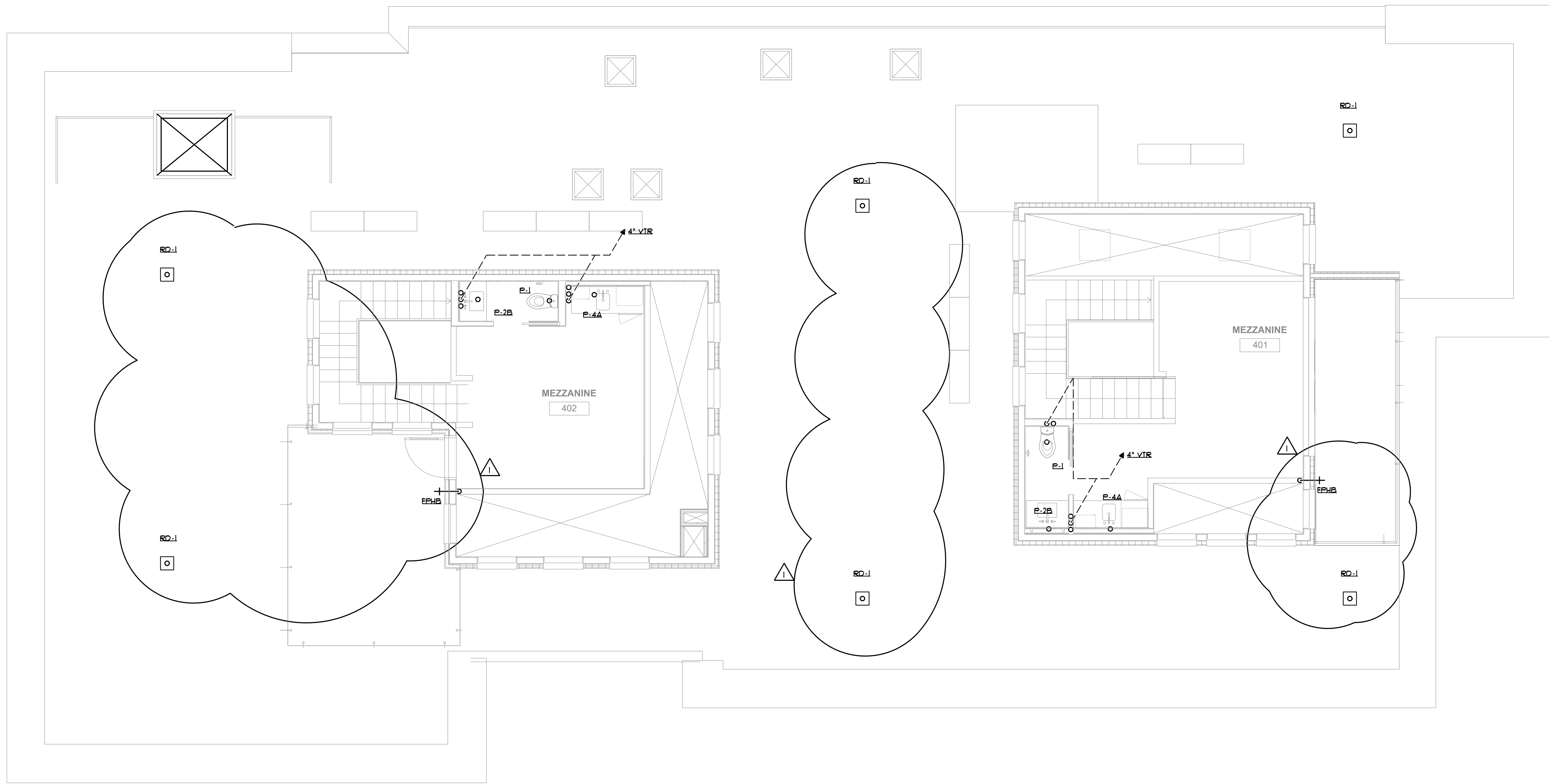
PENTHOUSE/ROOF PLUMBING PLAN SCALE - 1/4" = 1'-0"
