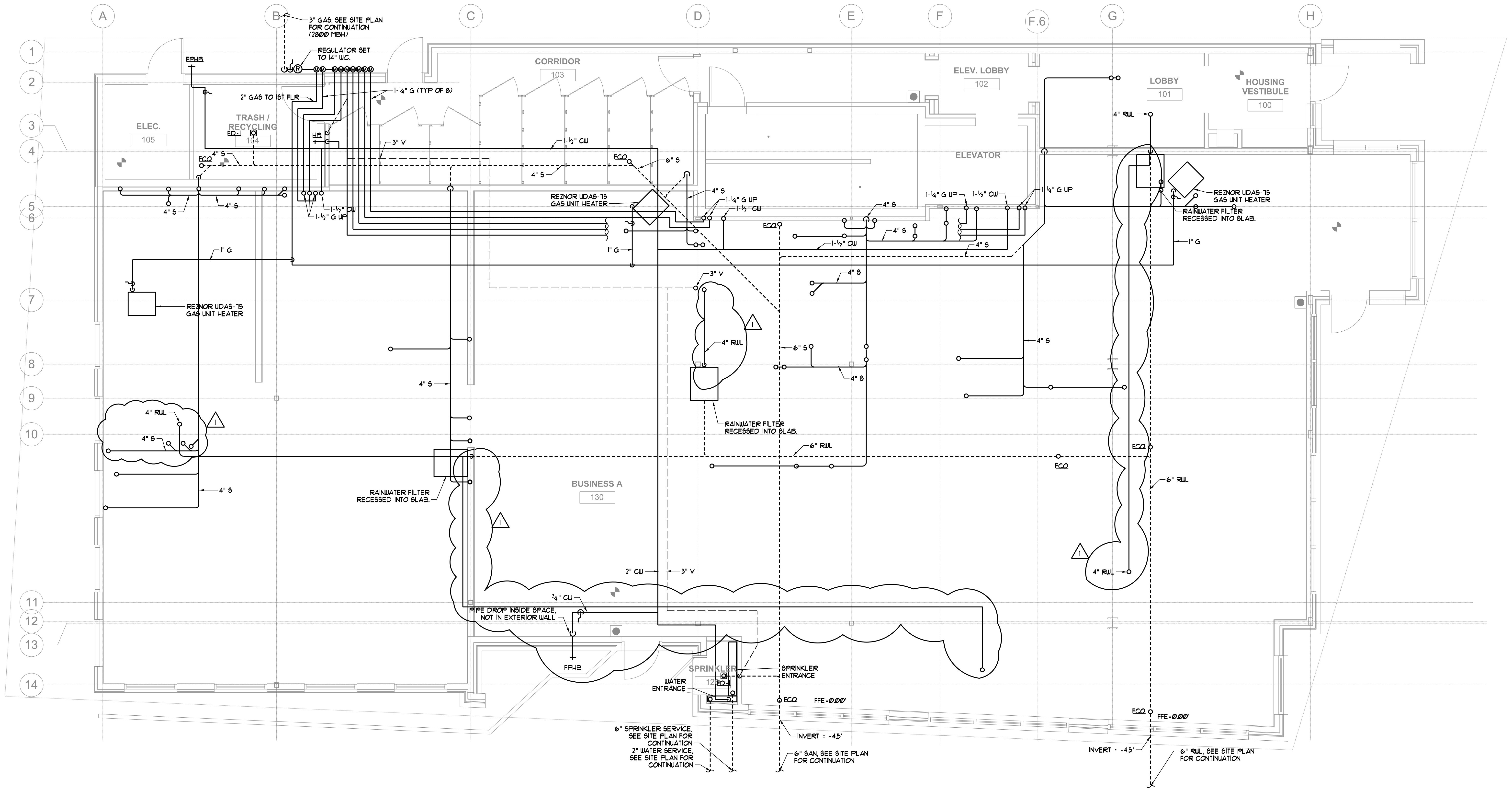
FIRST FLOOR PLUMBING PLAN SCALE - 1/4" = 1'-0"
