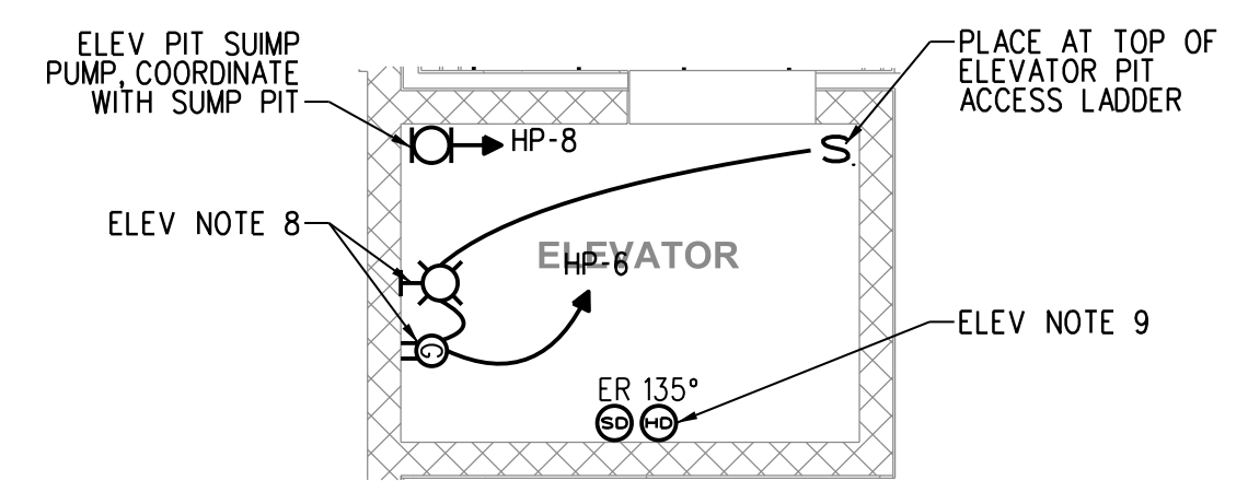
ELEVATOR PIT DETAIL SCALE: 1/4" = 1'-0" REFER TO DRAWING E3.0 FOR ELEVATOR NOTES
