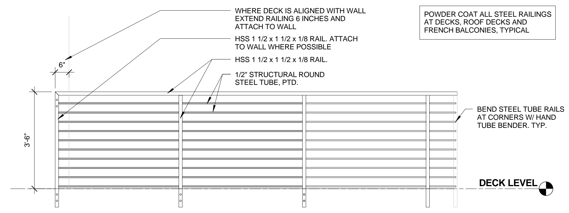
7 | TYPICAL DECK RAIL ELEVATION 1/2" = 1'-0"
