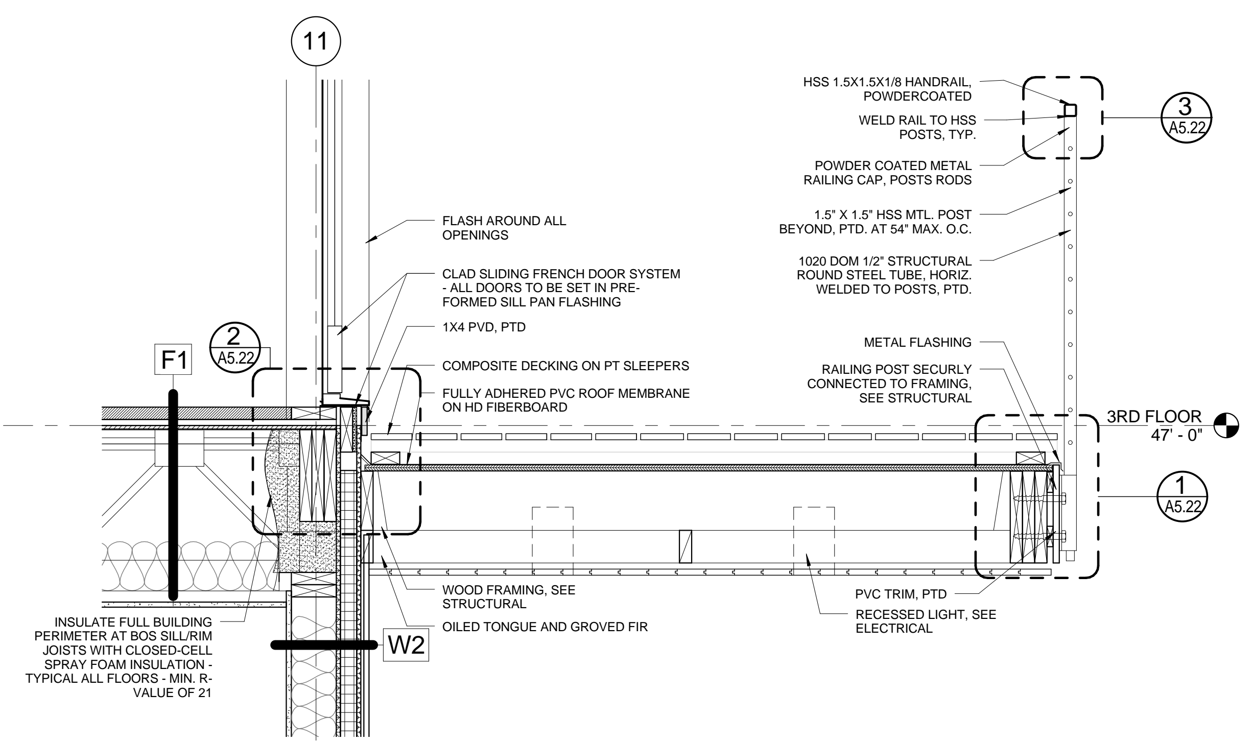
6 | TYP. DETAIL AT BALCONIES 1" = 1'-0"
