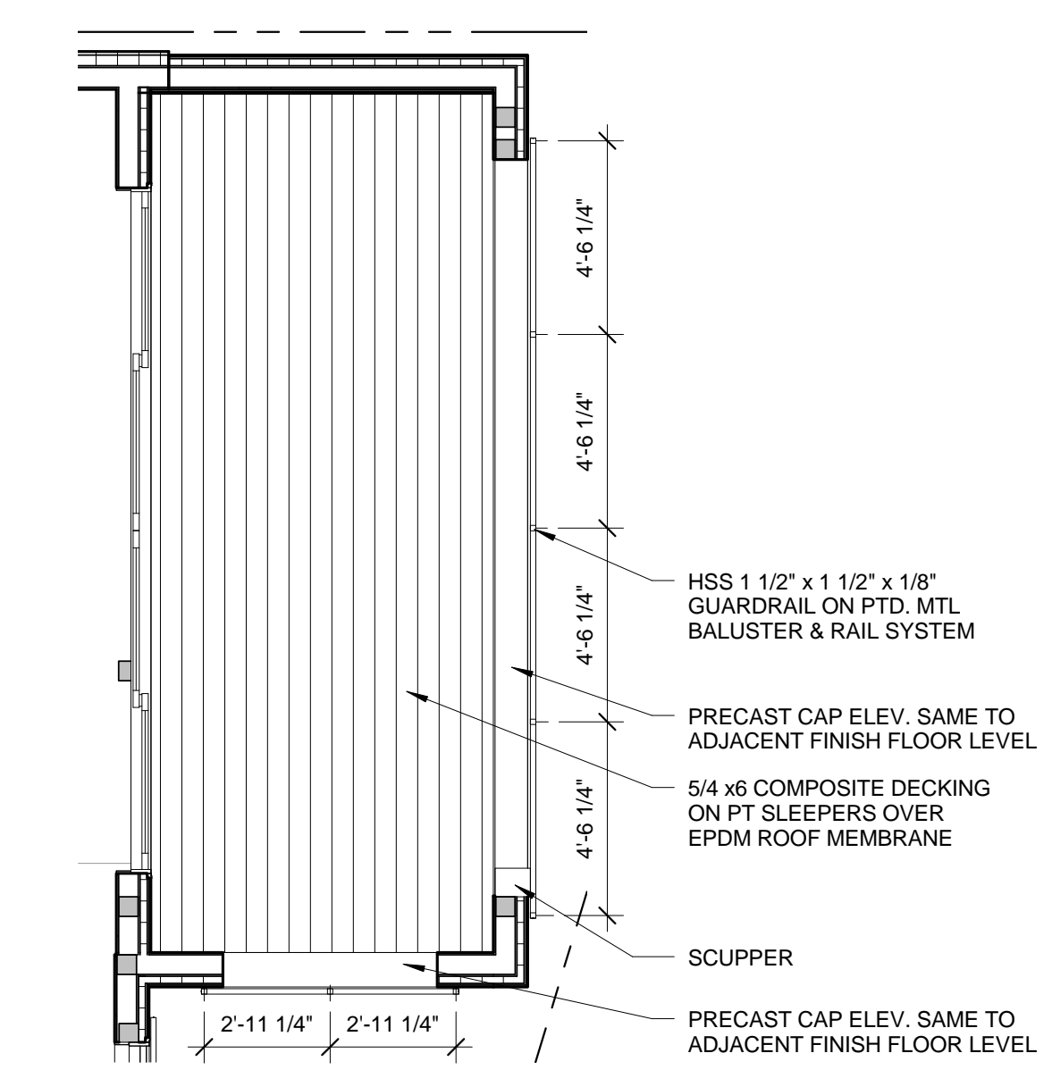
1. | DECK AT UNIT 401 1/4" = 1'-0"
