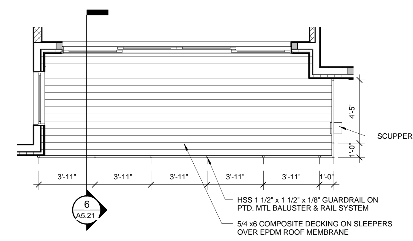
3 | DECK AT UNIT 402 1/4" = 1'-0"
