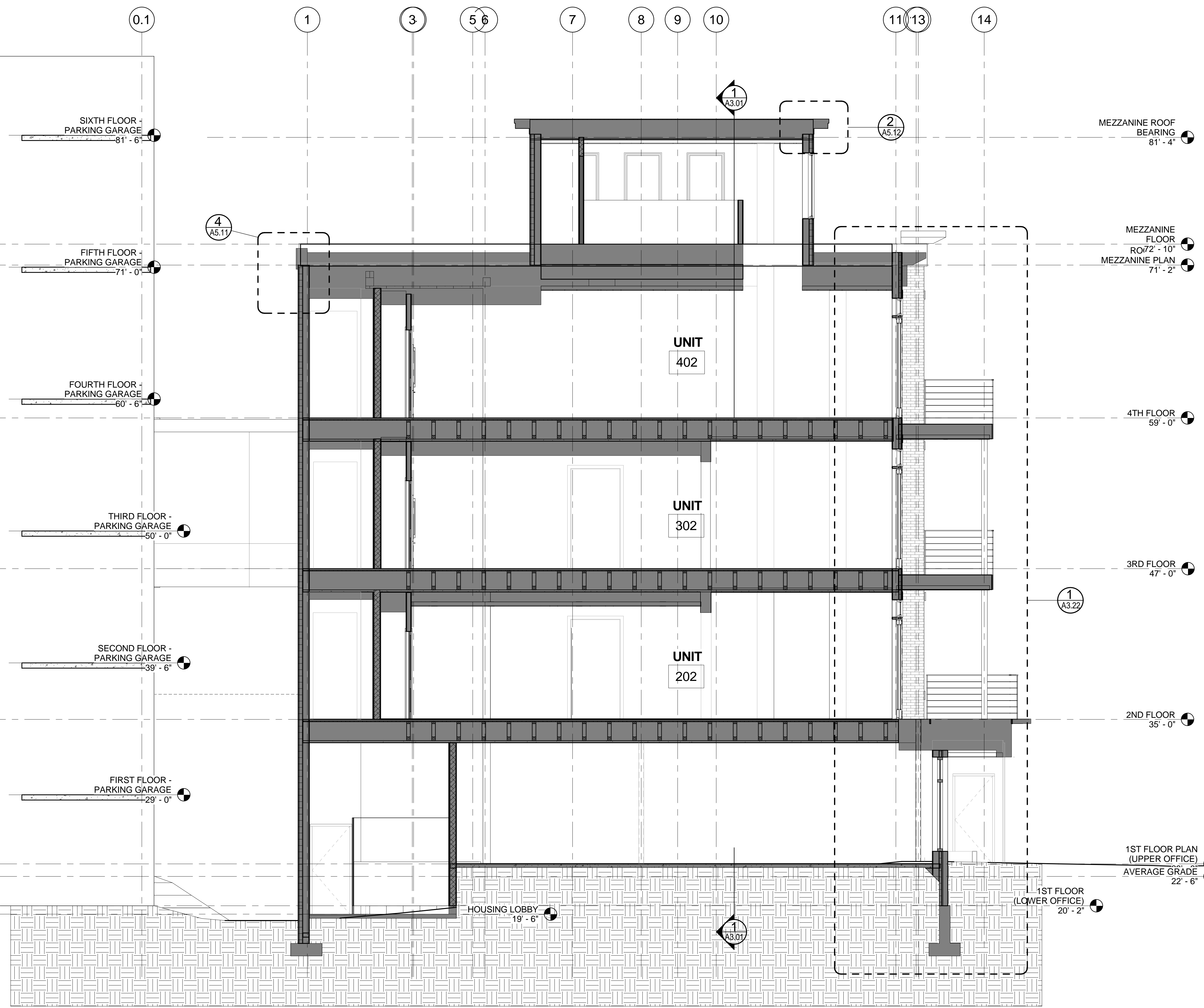
1 | N-S SECTION 1/4" = 1'-0" 0 1'-0" 2'-0" 4'-0" 8'-0"
