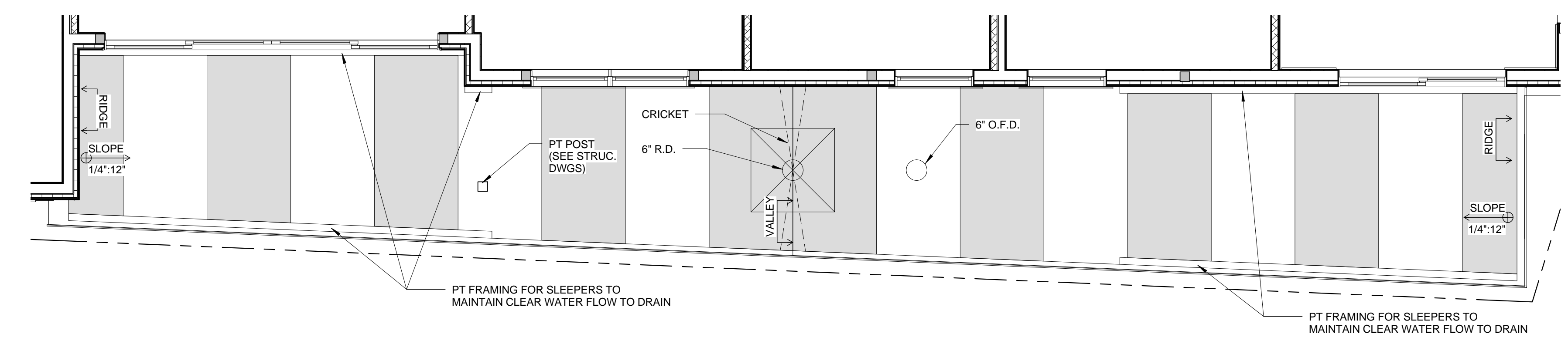
2 | SECOND FLOOR DECK TAPERED INSULATION 1/4" = 1'-0" 0 1'-0" 2'-0" 4'-0" 8'-0"
