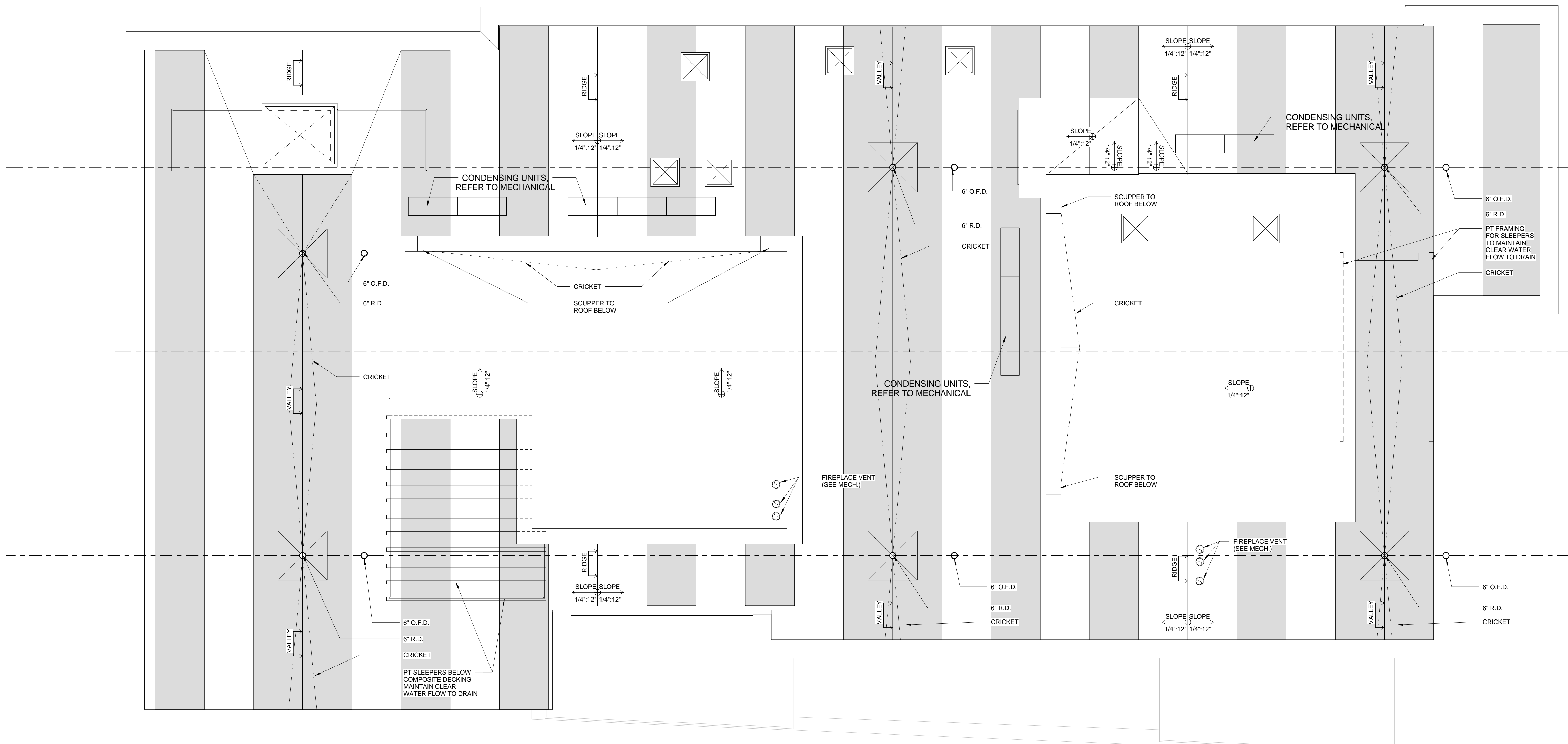
1 | ROOF MEZZANINE TAPERED INSULATION 1/4" = 1'-0" 0 1'-0" 2'-0" 4'-0" 8'-0"
