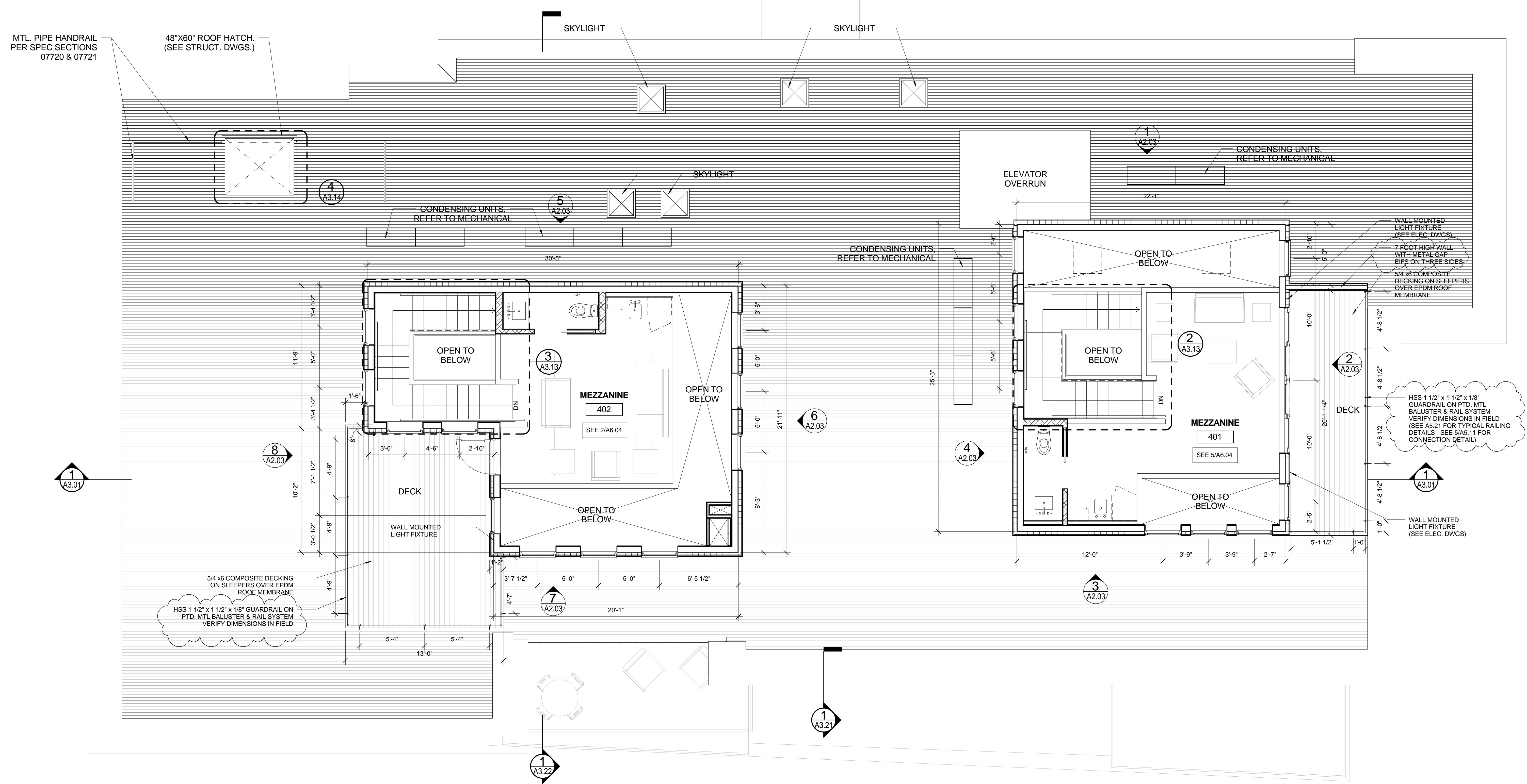
1 | ROOF AND MEZZANINE PLAN 1/4" = 1'-0"
