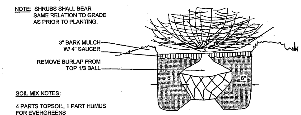
PLANTING DETAIL - SHRUB N.T.S.
