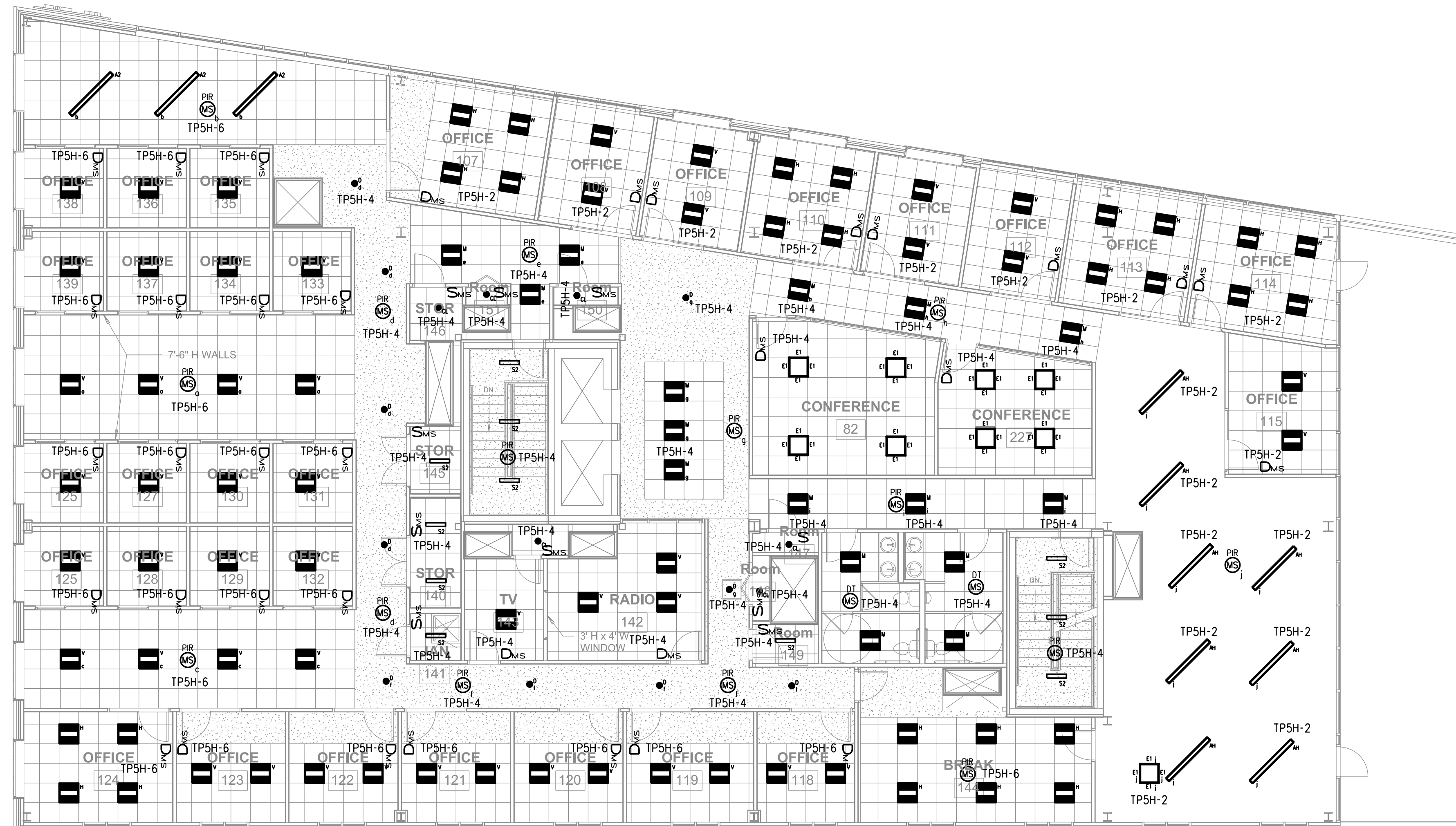
LIGHTING PLAN SCALE: 1/8" = 1'-0"
