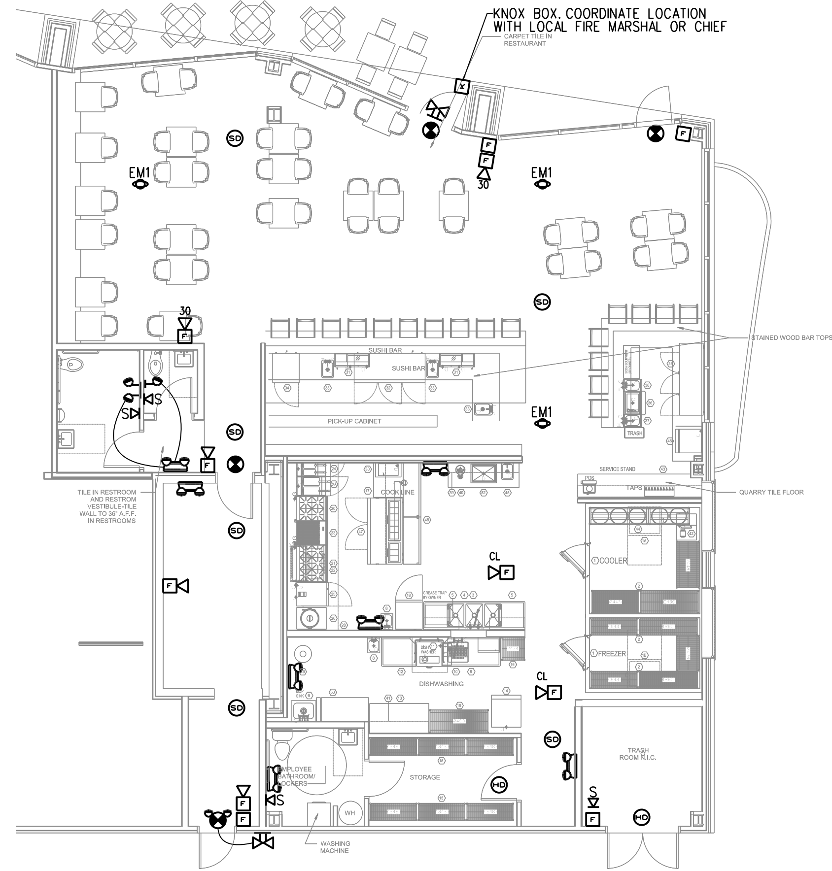
FIRST FLOOR RESTAURANT LIFE SAFETY PLAN SCALE: 1/8" = 1'-0"
