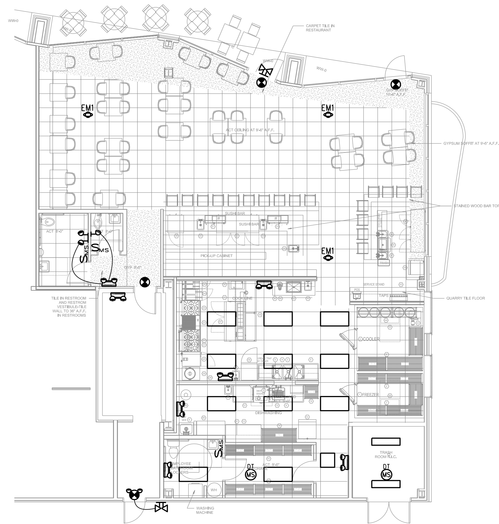
FIRST FLOOR RESTAURANT LIGHTING PLAN SCALE: 1/8" = 1'-0"
