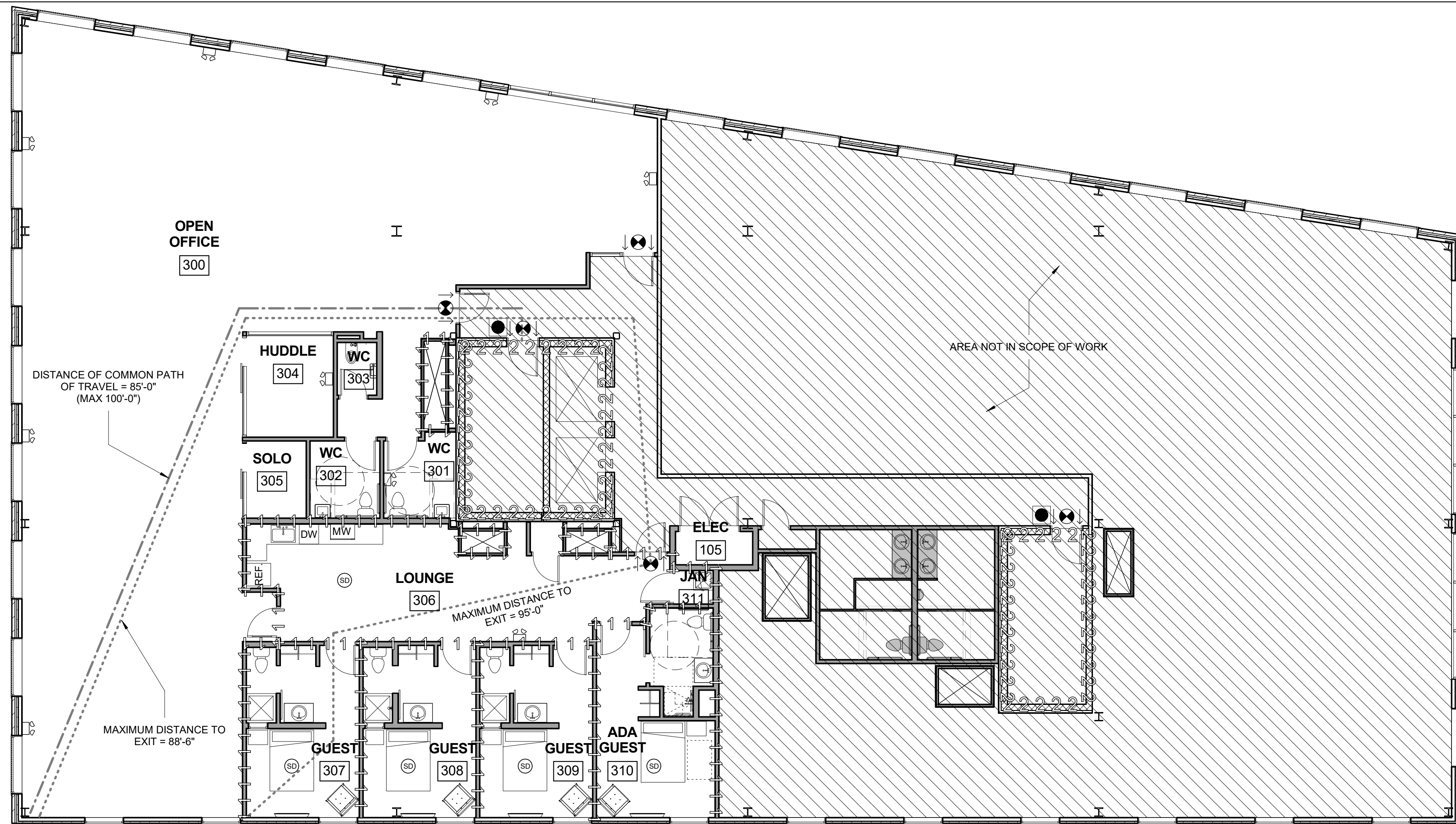
1 | TILSON 3RD FLOOR LIFE SAFETY PLAN 1/8" = 1'-0"
