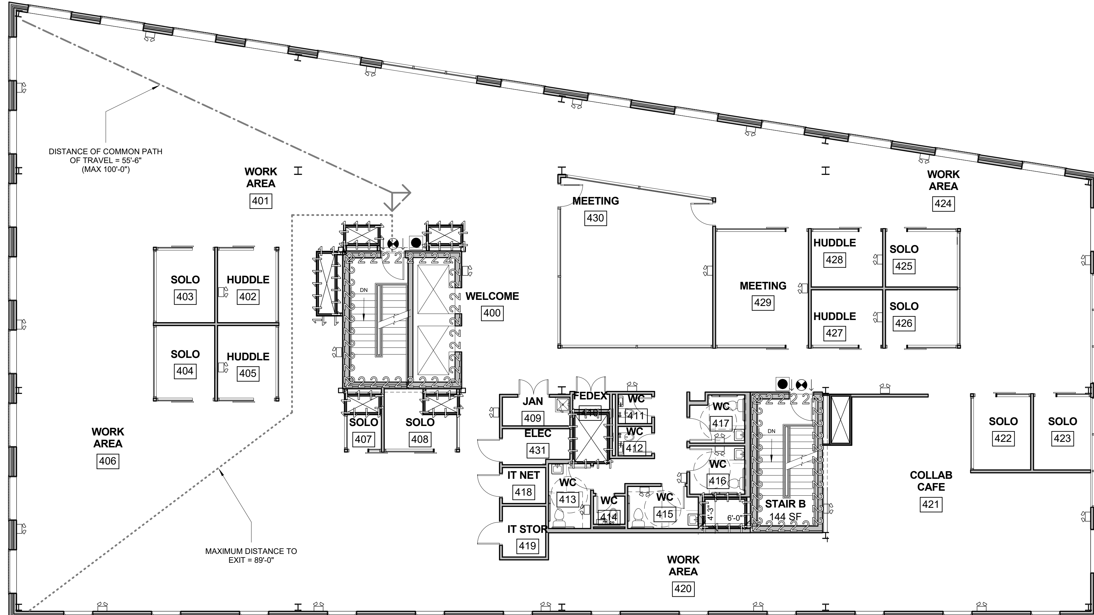
2 | TILSON 4TH FLOOR LIFE SAFETY PLAN
