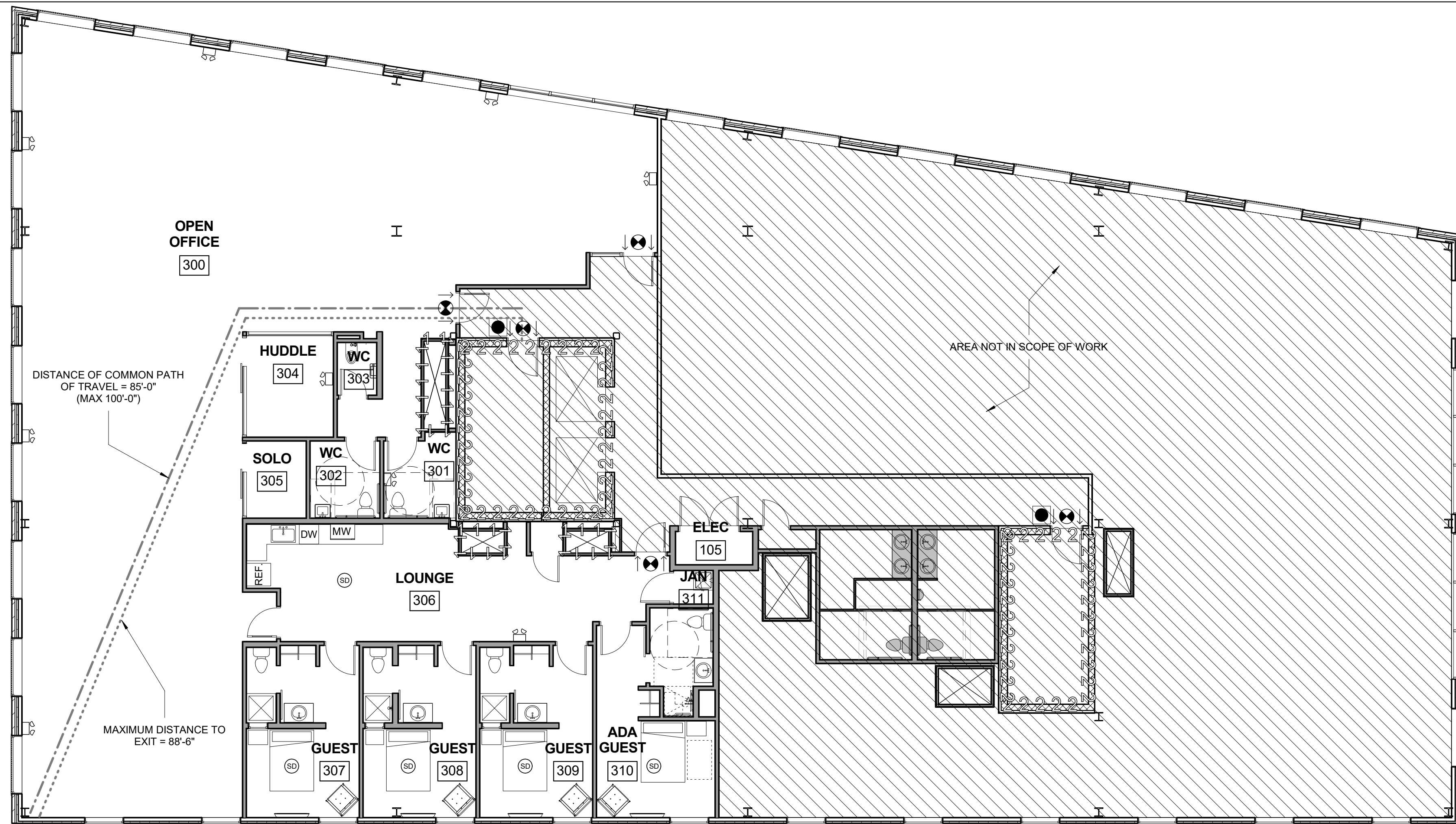
1 | TILSON 3RD FLOOR LIFE SAFETY PLAN
