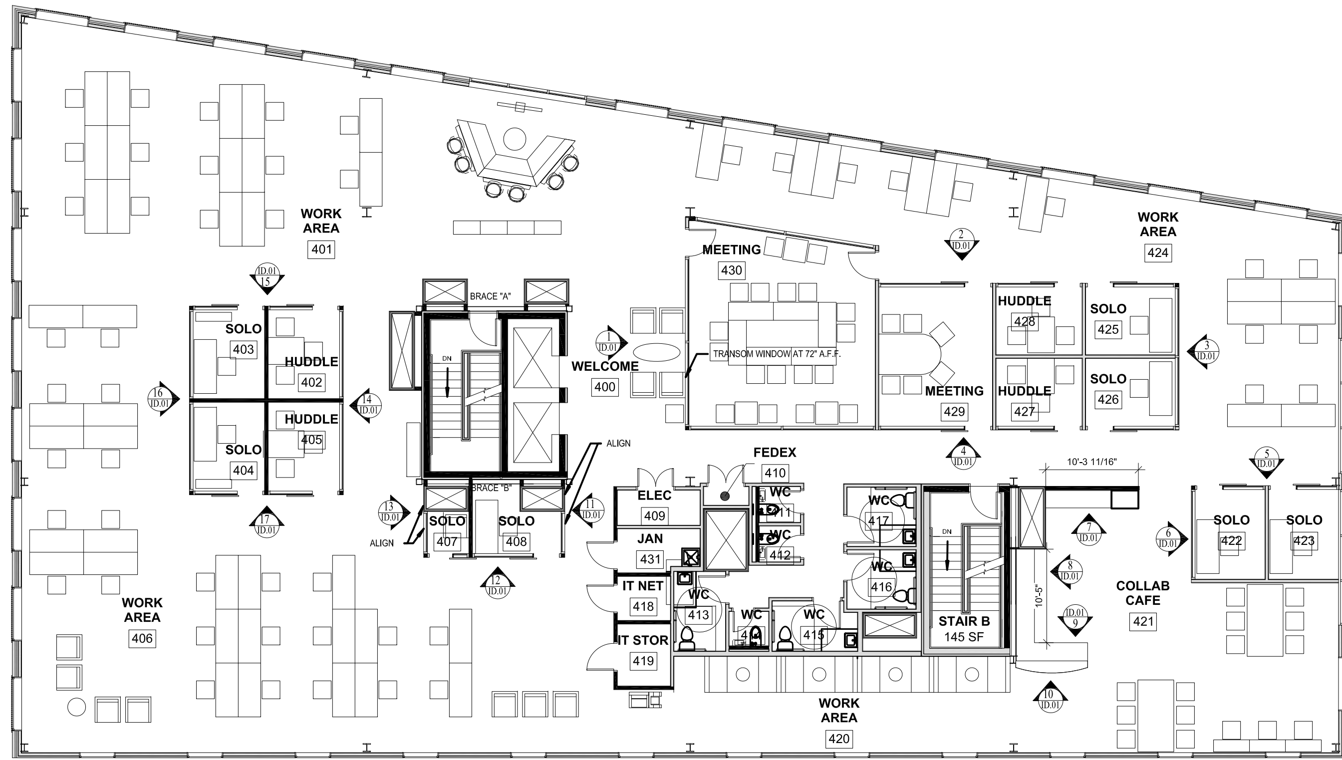
1 | TILSON 4TH FLOOR PLAN 1/32" = 1'-0"
