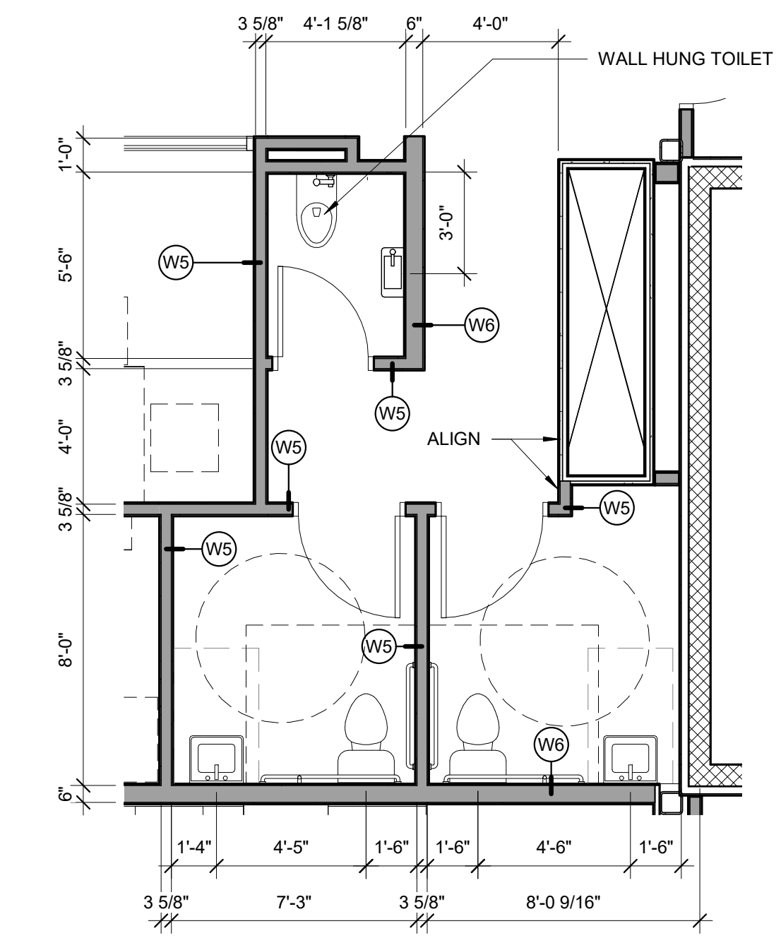
4 TILSON RESTROOM ENLARGED PLAN 1/4" = 1'-0"
