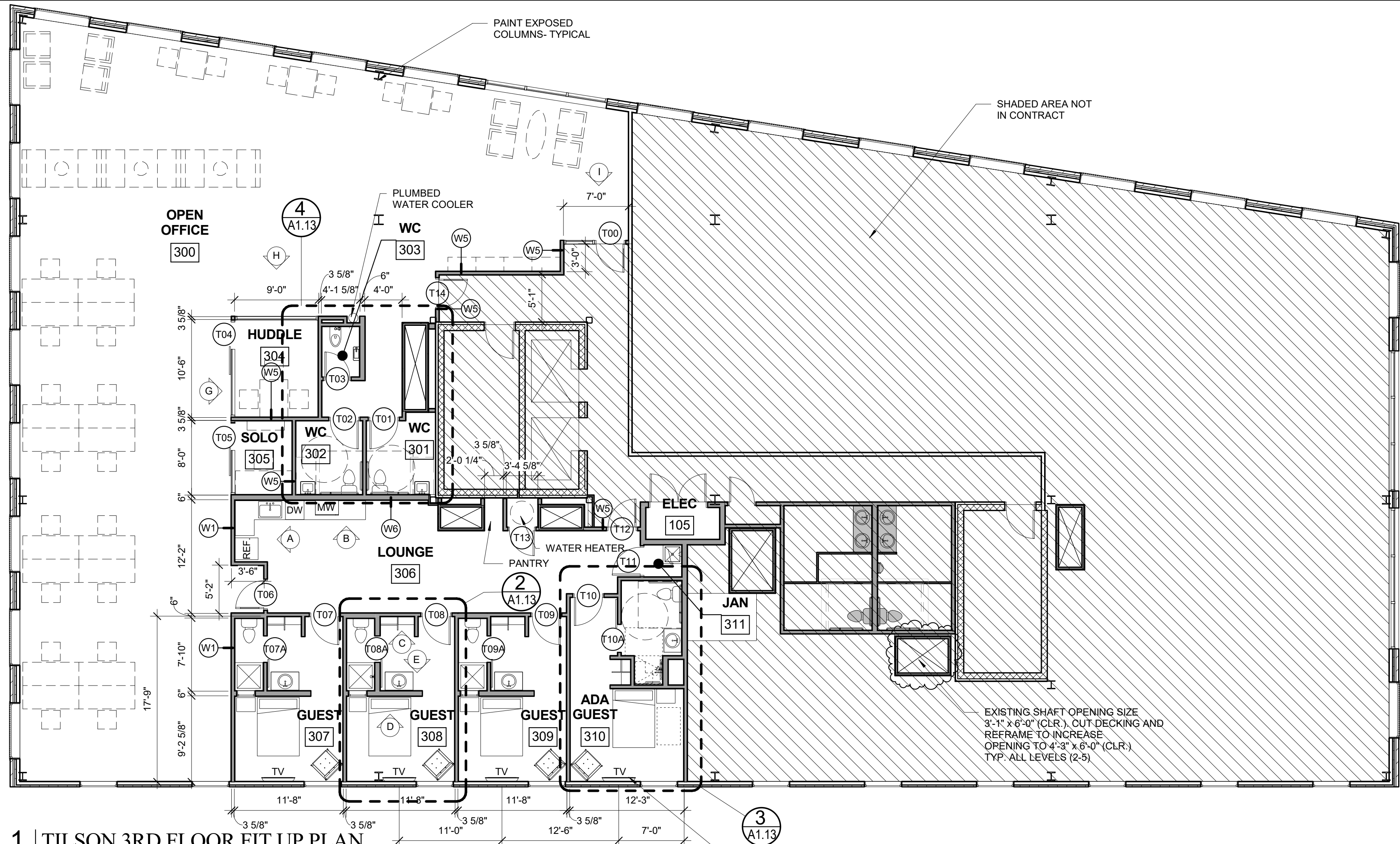
1 TILSON 3RD FLOOR FIT UP PLAN 1/8" = 1'-0"
