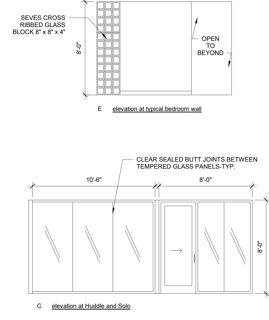
6 3rd floor elevations 1/4" = 1'-0"
