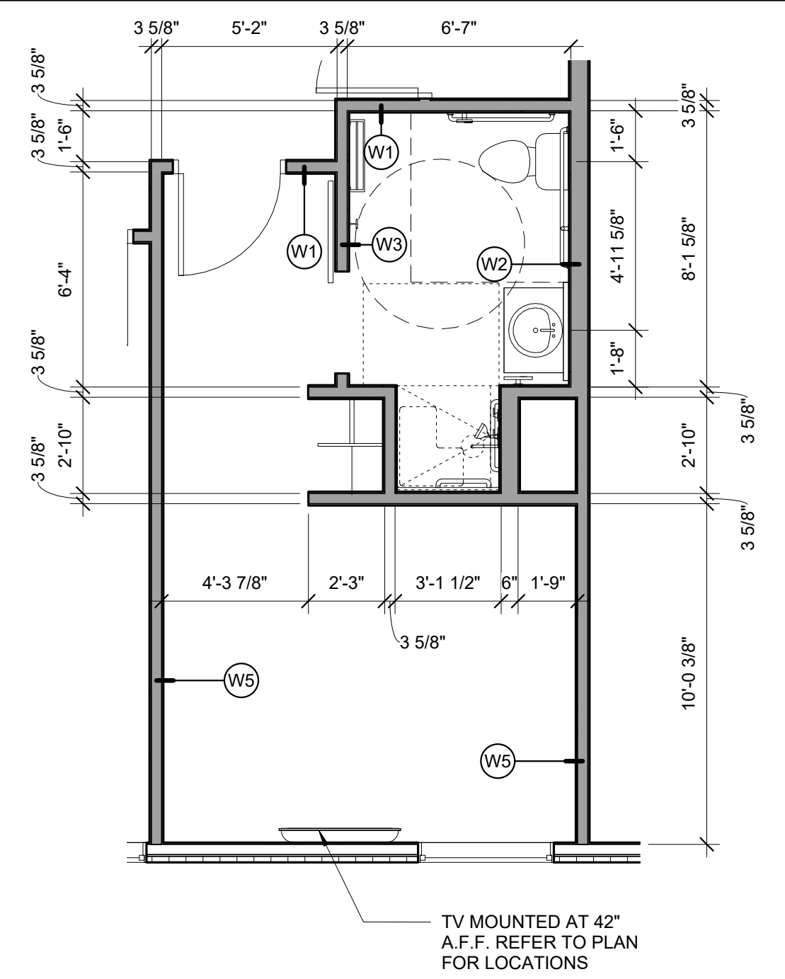
3 TILSON ADA GUEST ROOM ENLARGED PLAN 1/4" = 1'-0"
