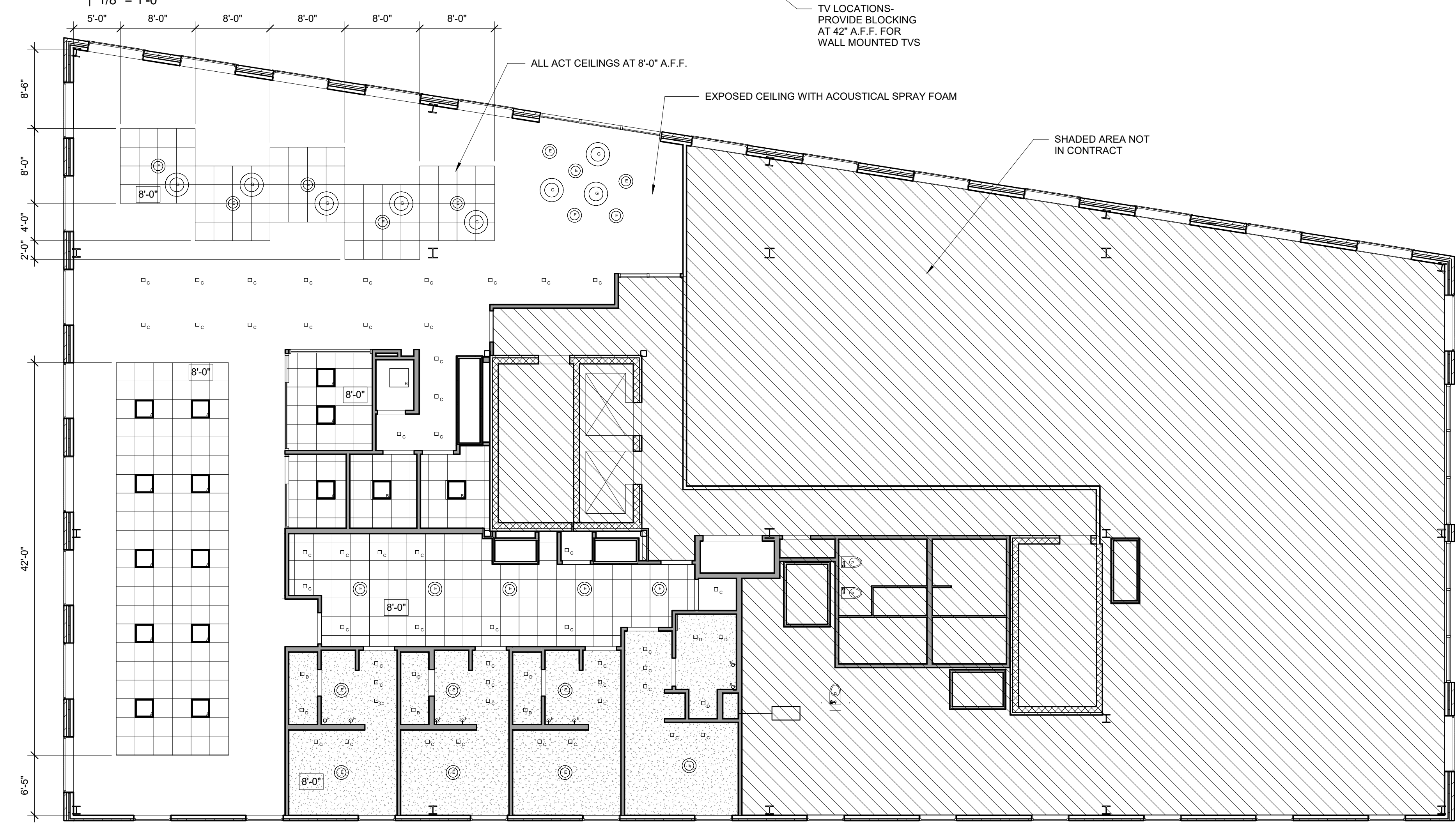
5 3RD FLOOR RCP 1/8" = 1'-0"
