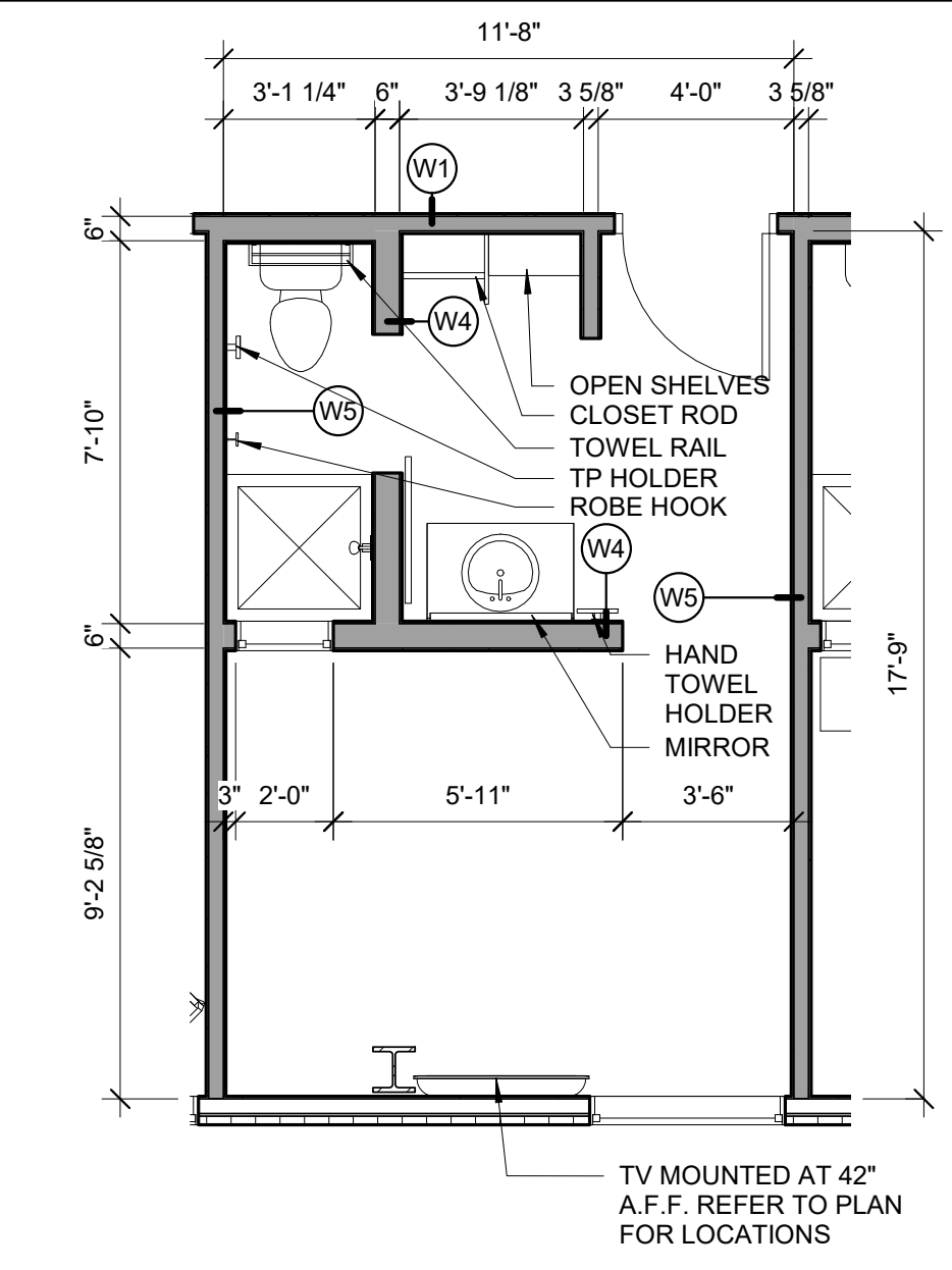
2 TYPICAL GUEST ROOM ENLARGED PLAN 1/4" = 1'-0"
