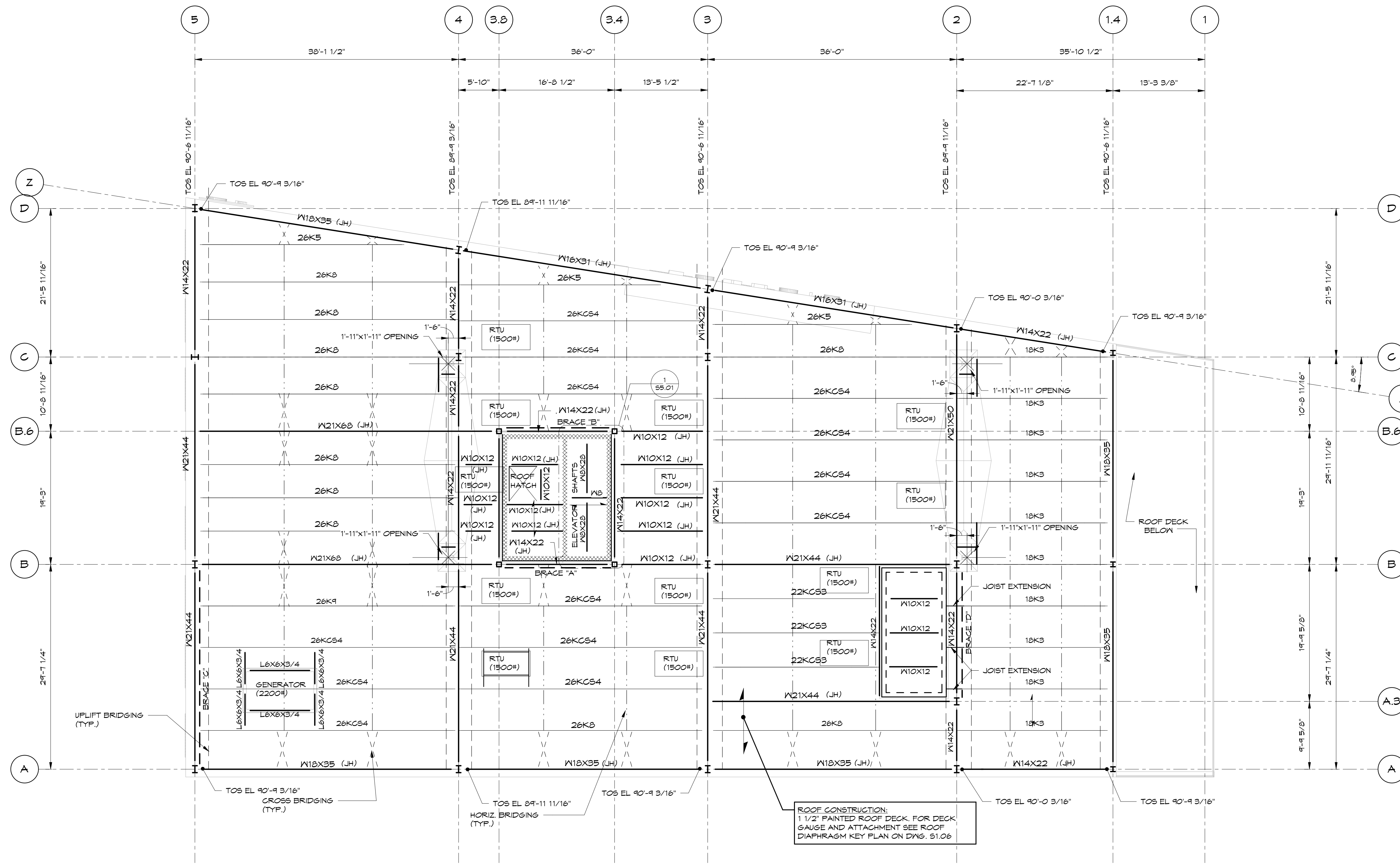
1 ROOF FRAMING PLAN 1/8" = 1'-0"
