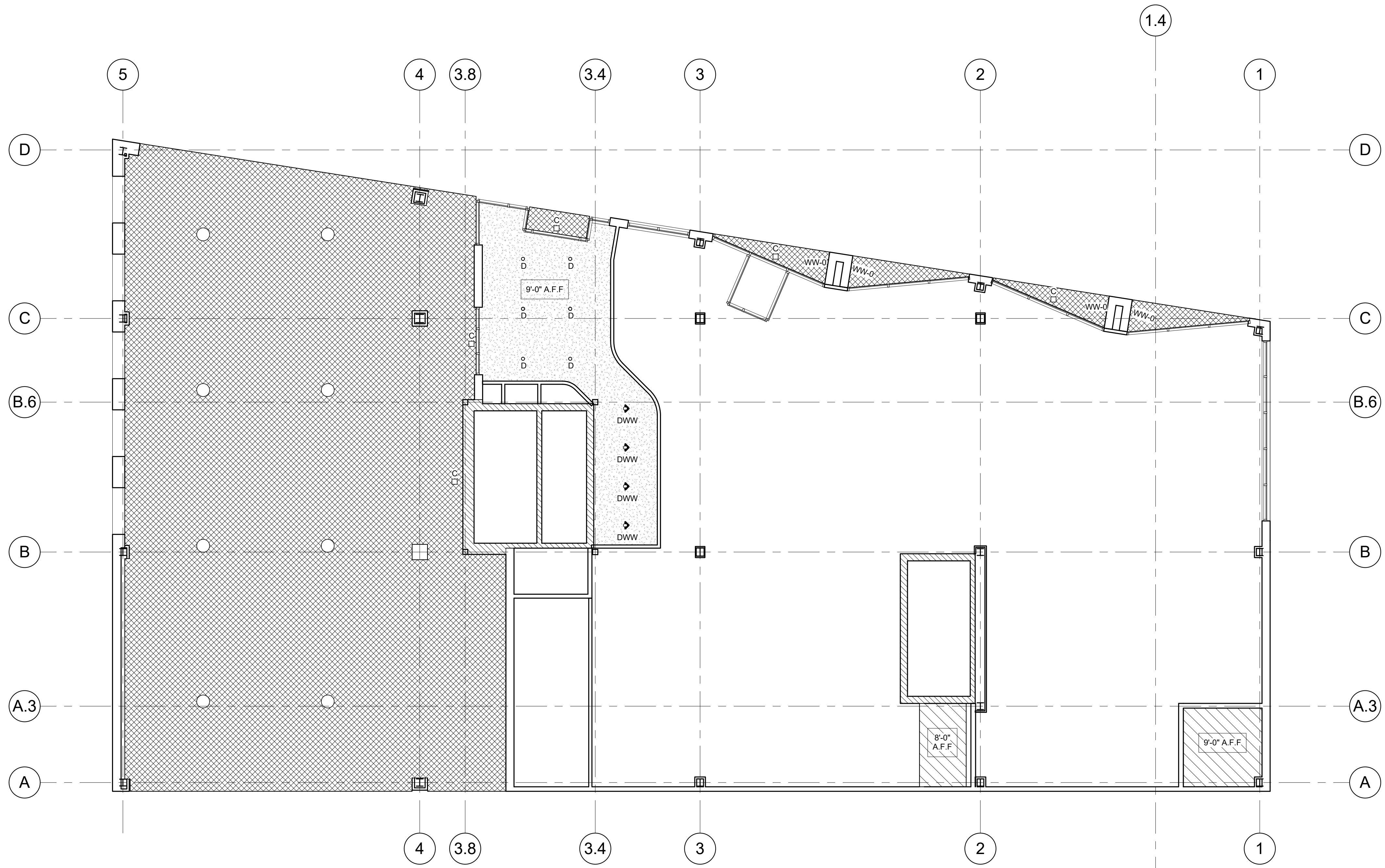
1 | 1ST FLOOR - LOBBY 1/8" = 1'-0"
