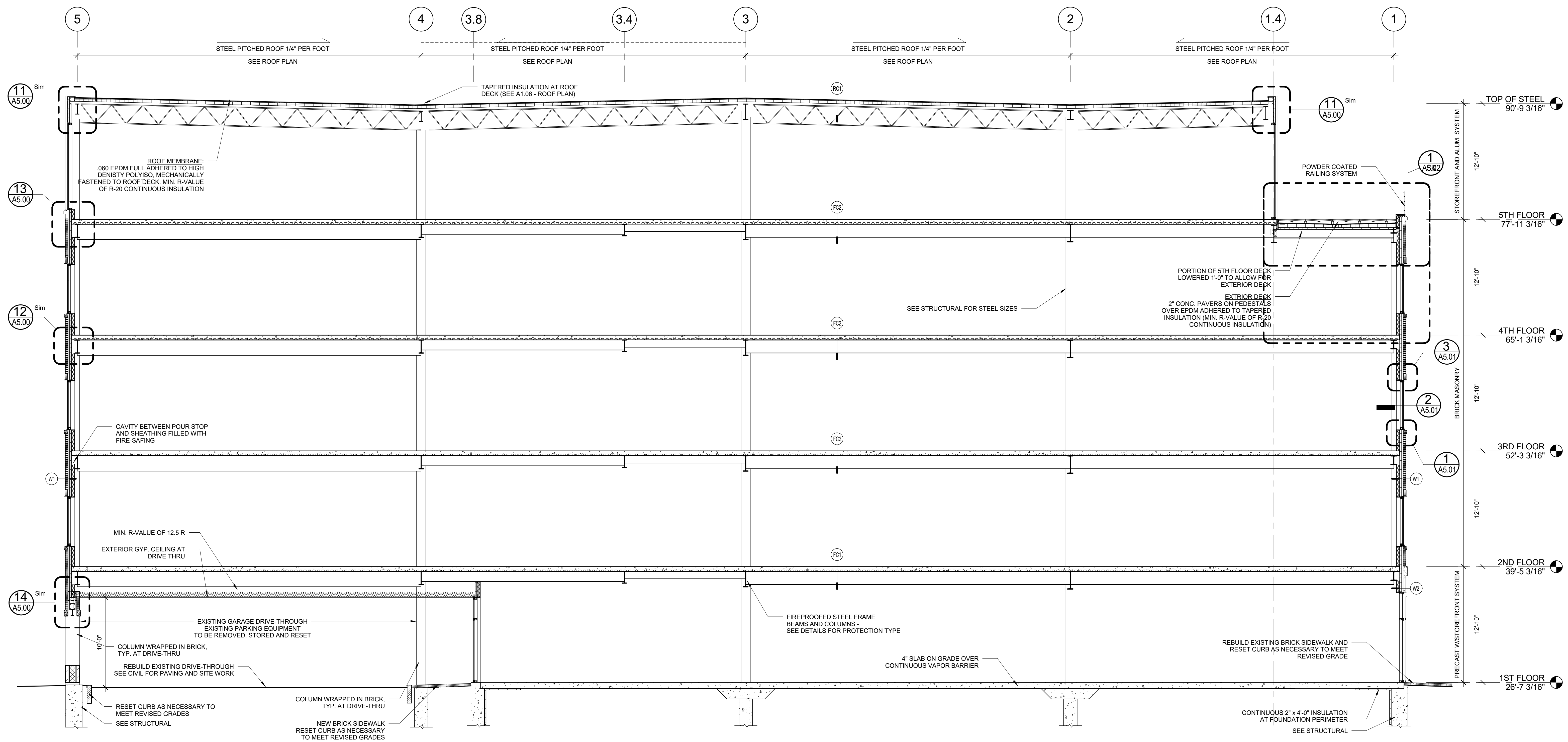
1 | BUILDING SECTION 3/16" = 1'-0"
