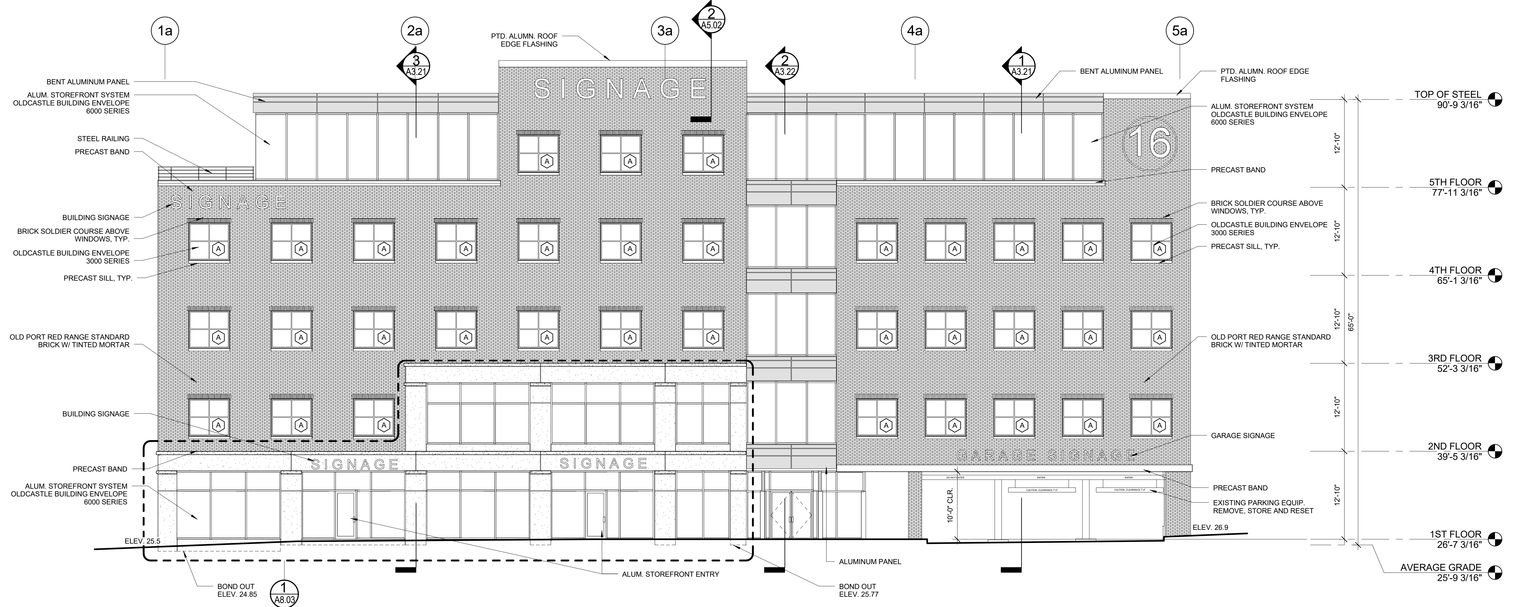
2 North Elevation 1/8" = 1'-0"
