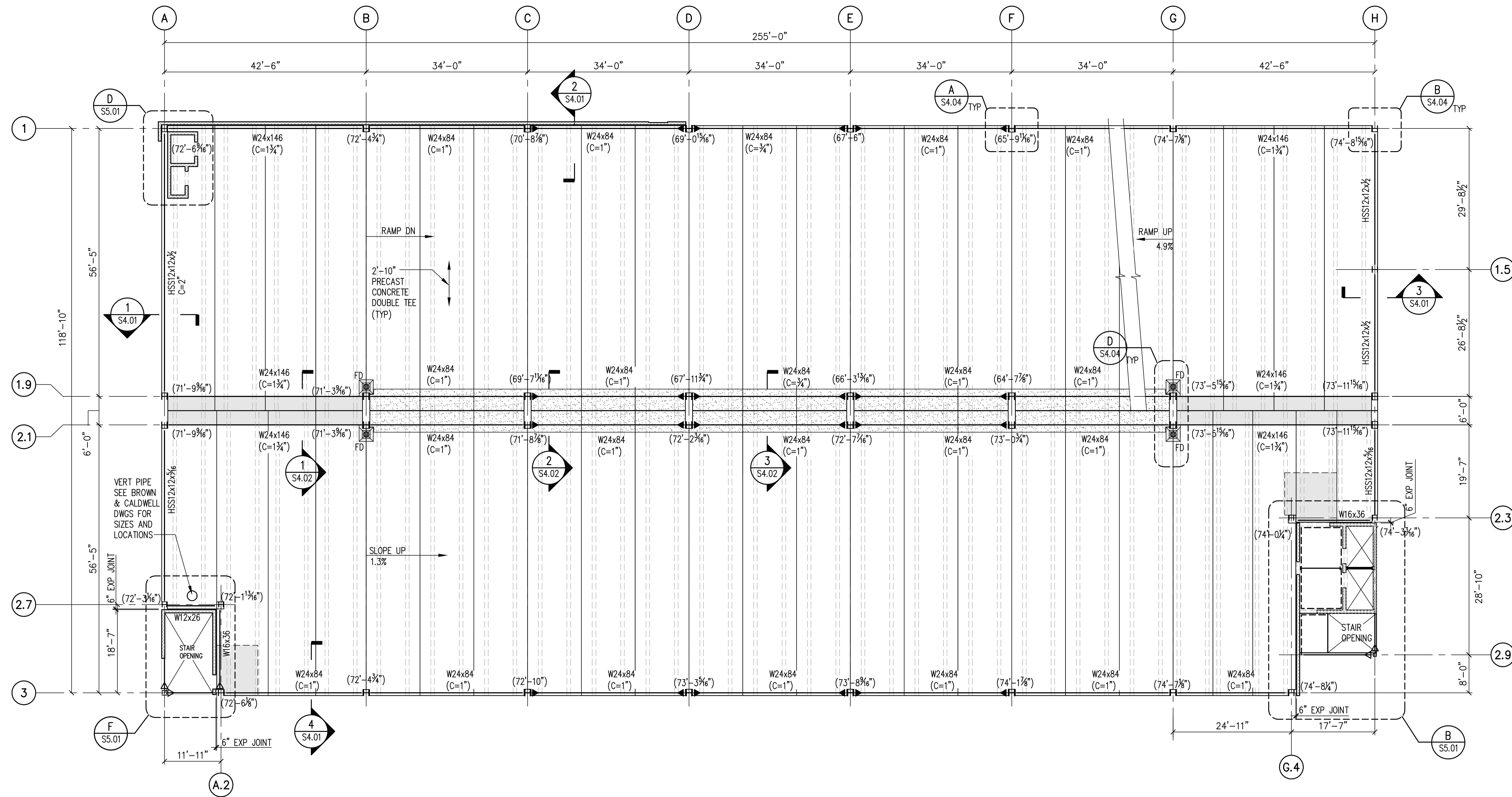
5TH FLOOR PLAN 3/32"=1'-0"
