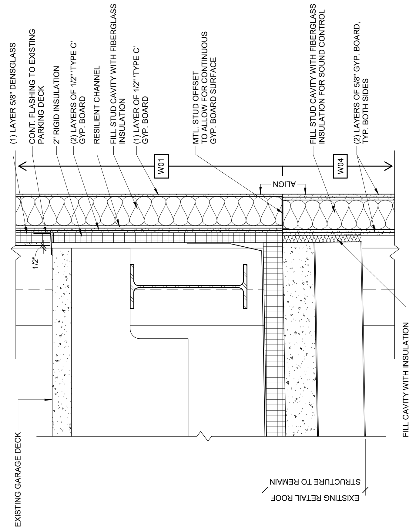
3 ELEVATOR SECTION BLOW UP 1" = 1'-0"
