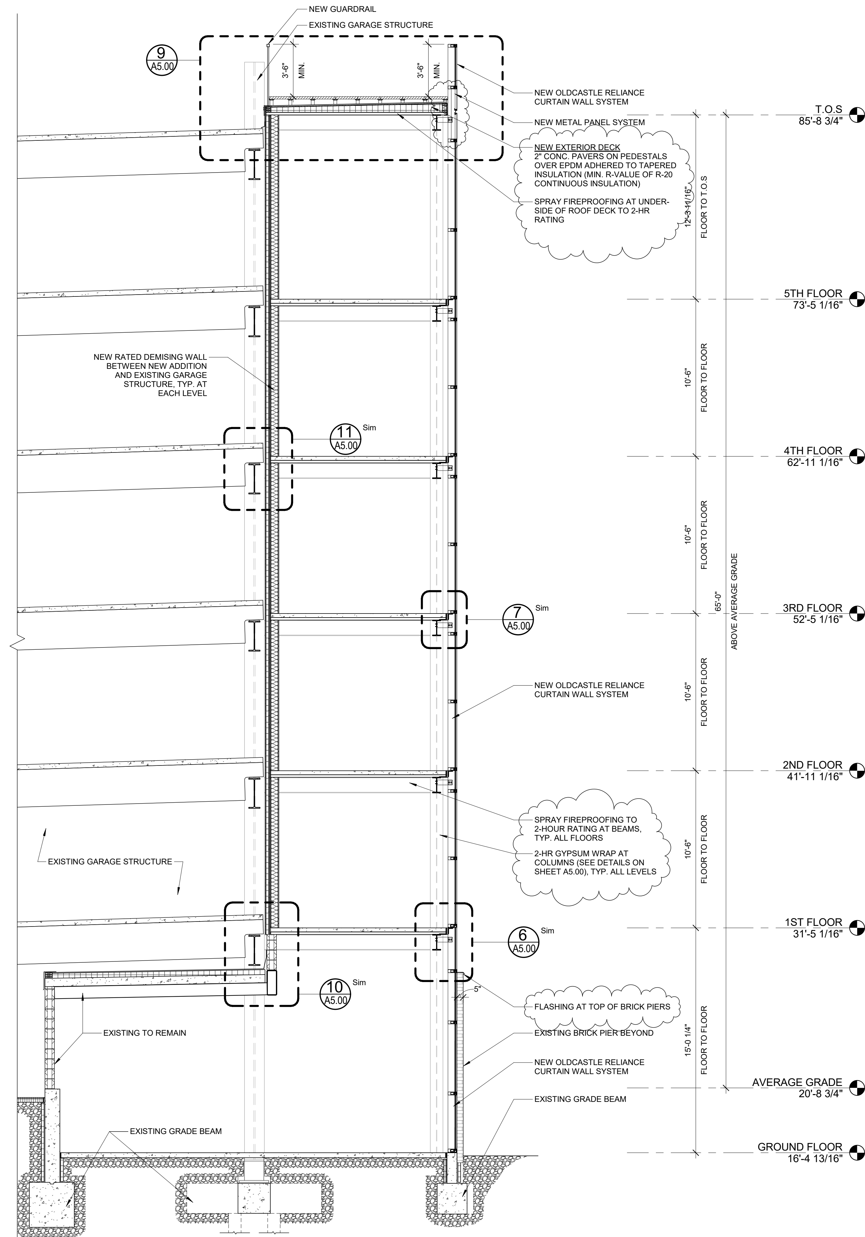
1 | CROSS SECTION THROUGH ADDITION 1/4" = 1'-0"
