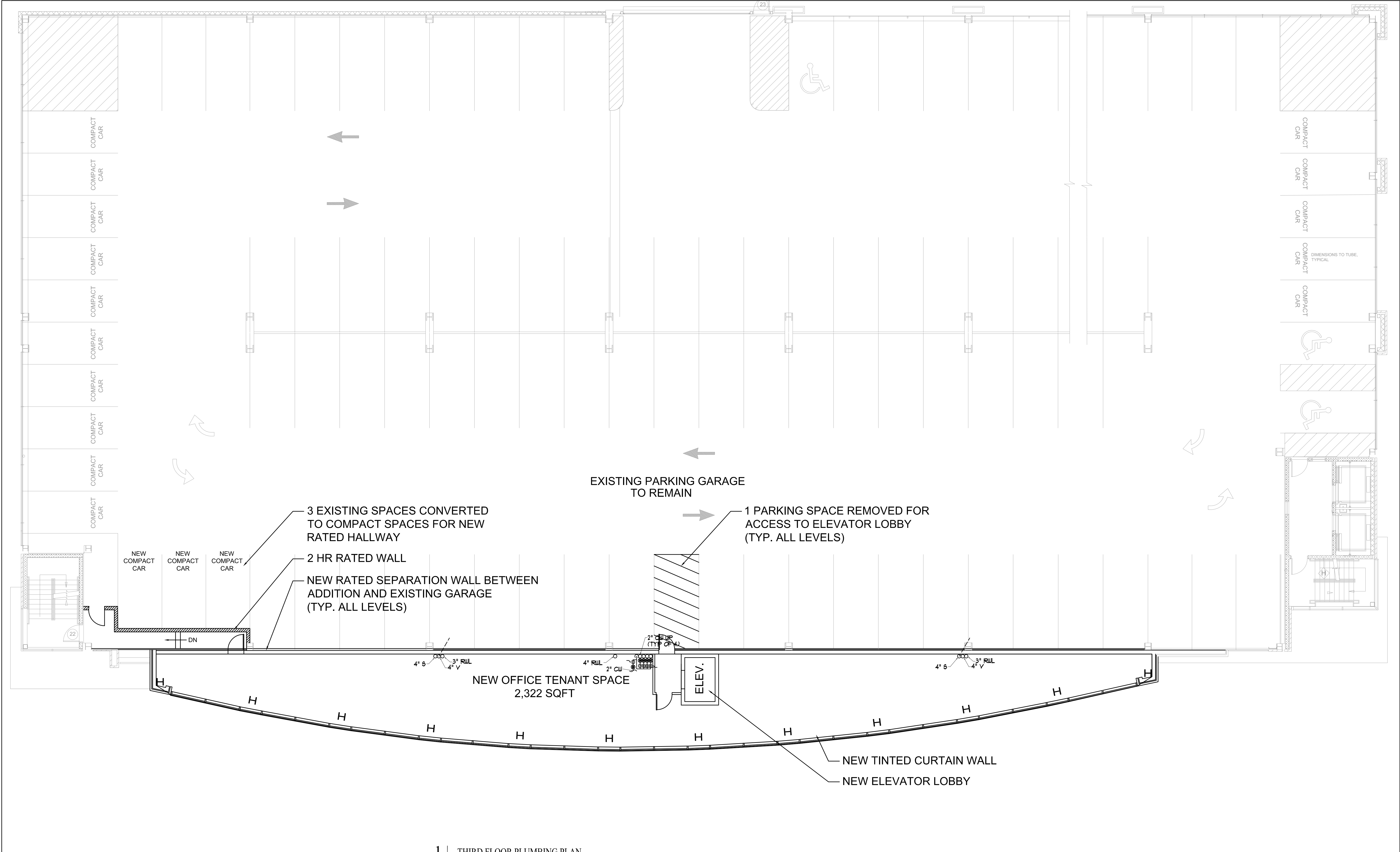
1 | THIRD FLOOR PLUMBING PLAN SCALE: 1/8"=1'-0"
