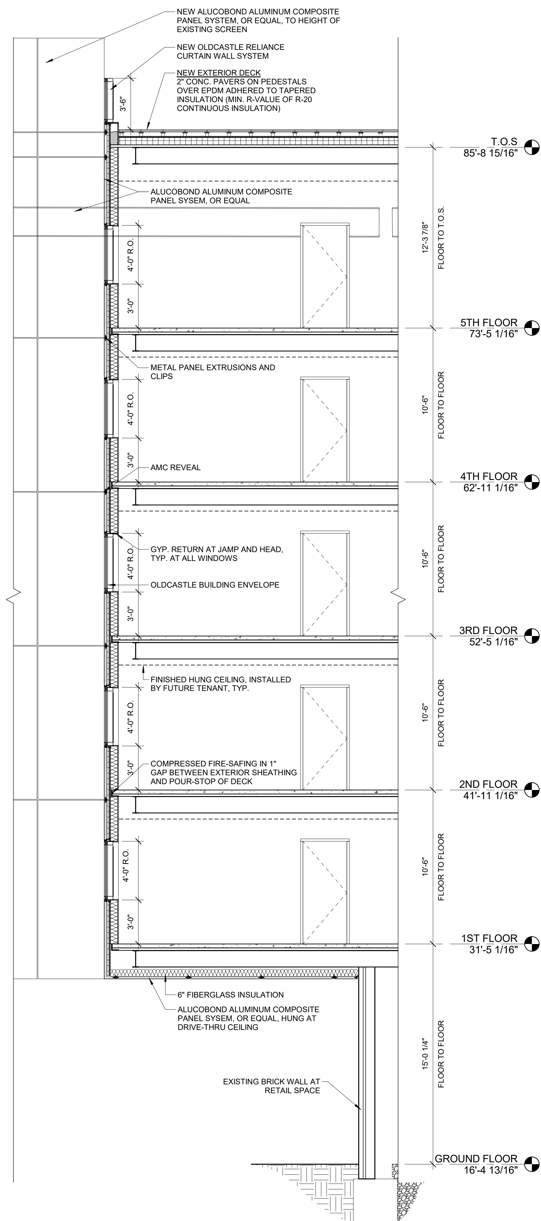
2 | SECTION THROUGH CANTILEVER END WALL 1/4" = 1'-0"
