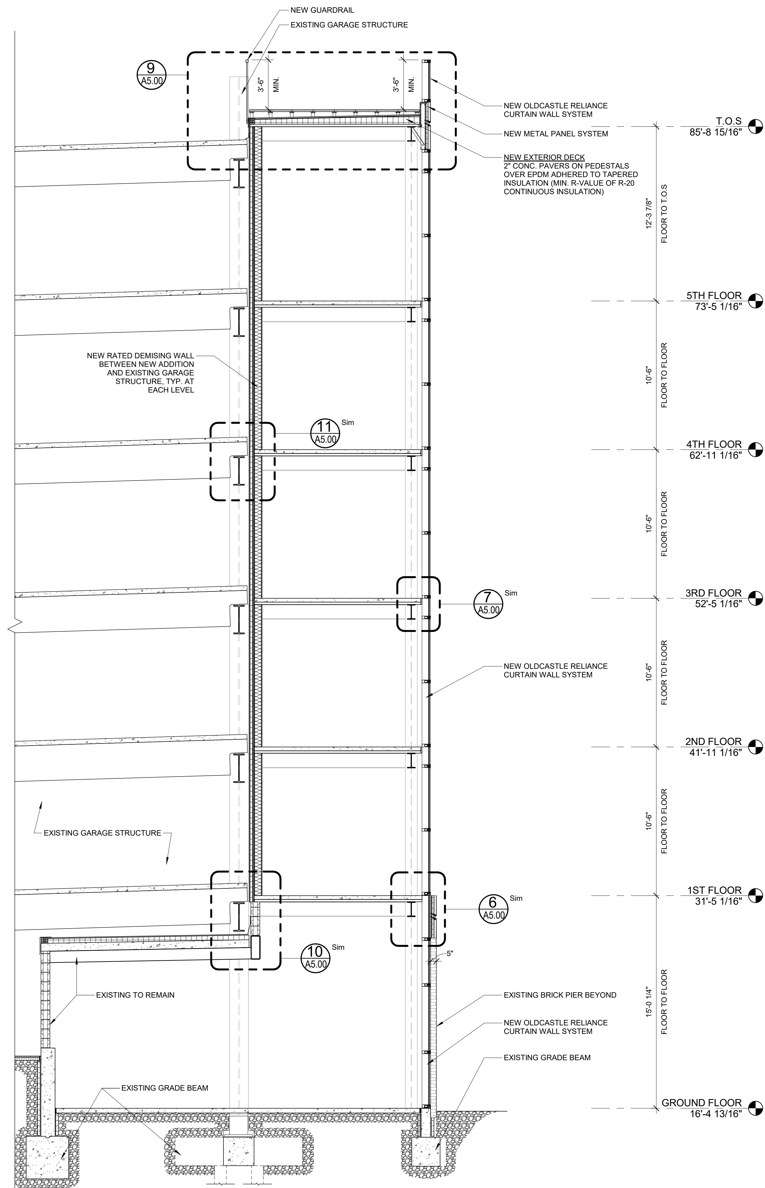
1 CROSS SECTION THROUGH ADDITION 1/4" = 1'-0"
