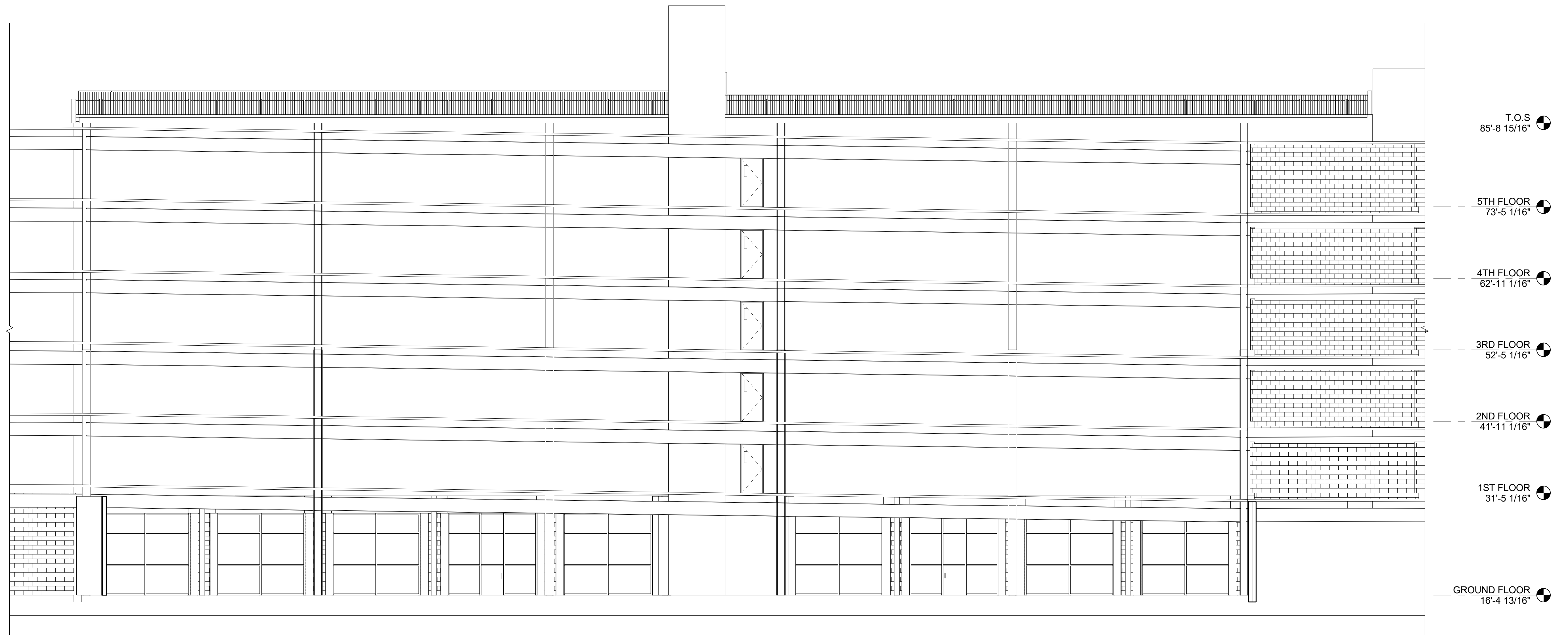
1 SECTION THROUGH EXISTING GARAGE 1/8" = 1'-0"
