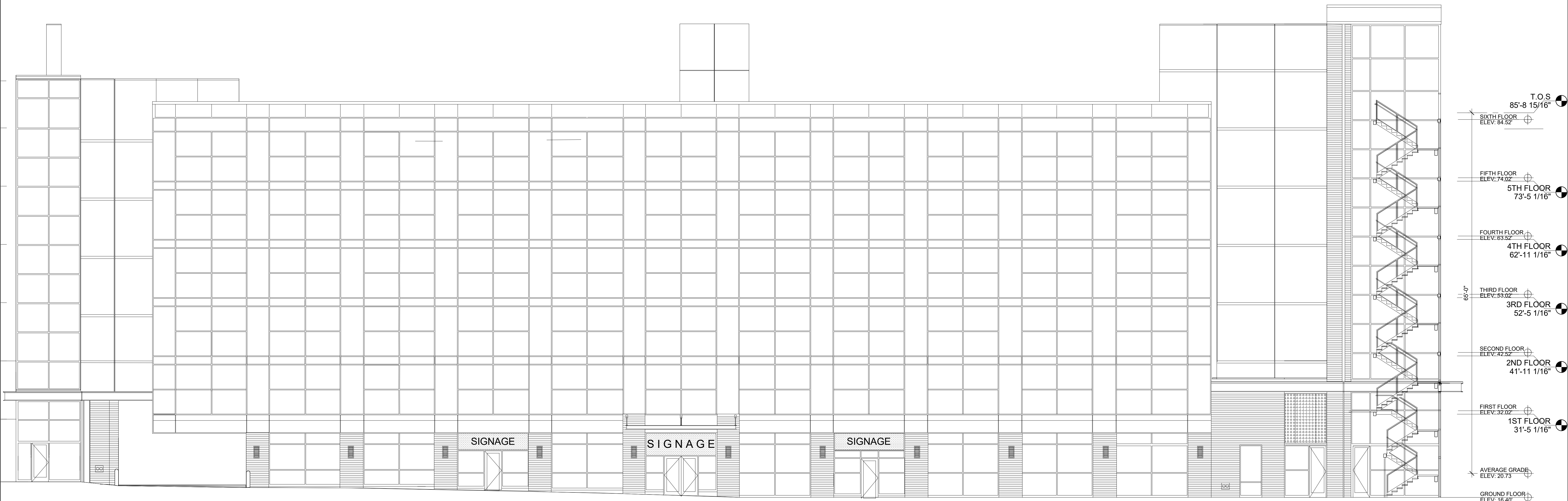
1 | FRONT ELEVATION 1/8" = 1'-0"
