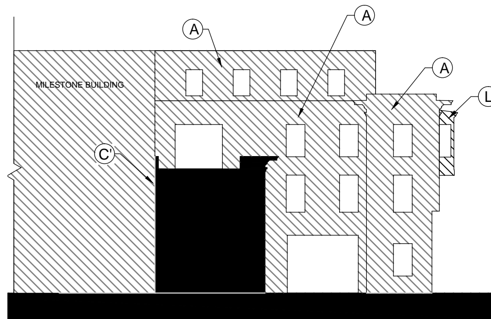
SOUTH-WEST ELEVATION
