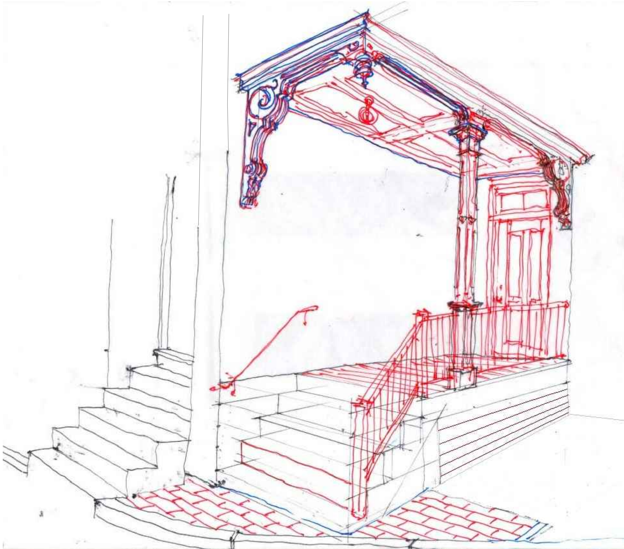
PROPOSED RESTORED ENTRY PORCH (NO SCALE)
