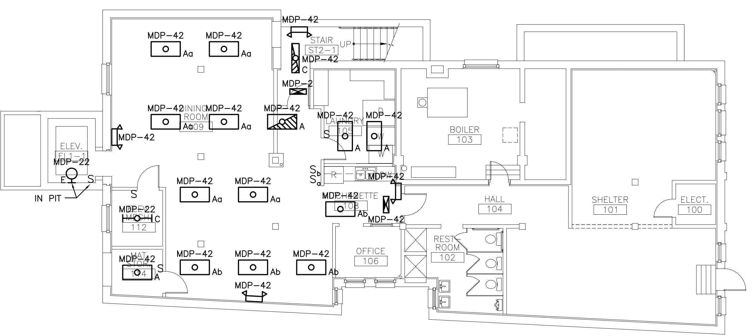
A1 FIRST FLOOR PLAN
