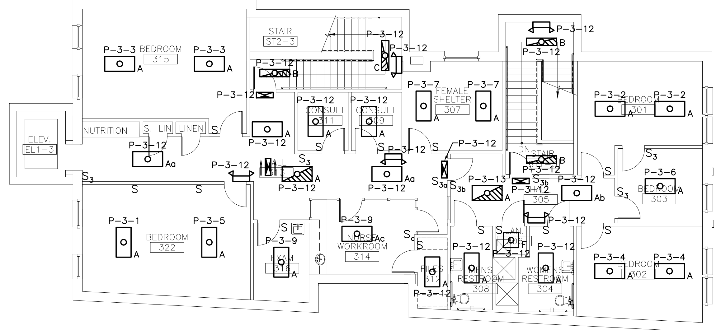
K1 THIRD FLOOR PLAN
