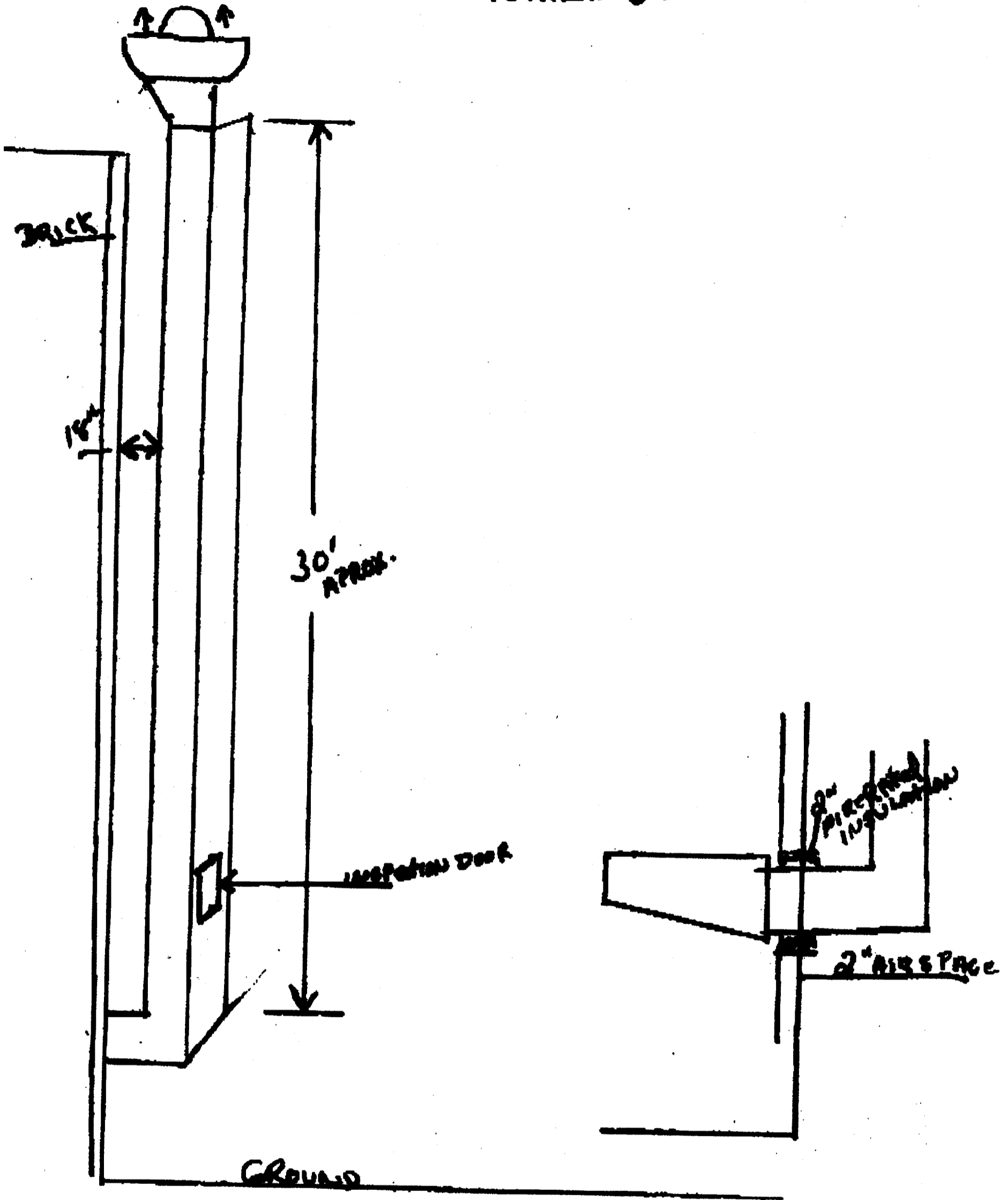
INSTALLATION of new Hood Fan.
