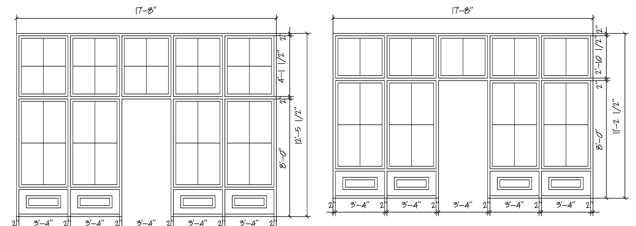
STOREFRONT TYPE A KAWNEER 061-222 2"x6" FRAME SYSTEM STOREFRONT TYPE B KAWNEER 061-222 2"x6" FRAME SYSTEM
