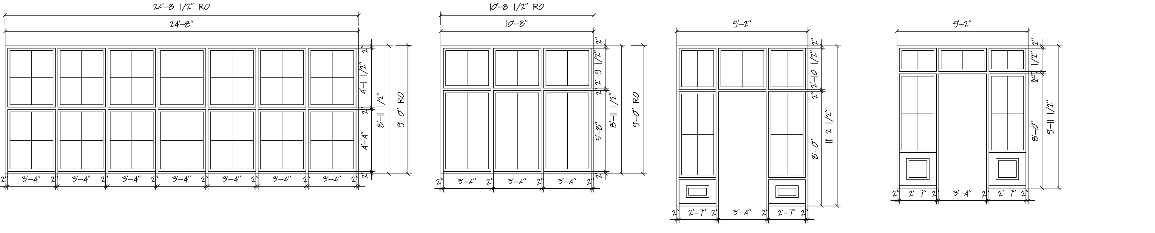
STOREFRONT TYPE C KAWNEER 061-222 2"x6" FRAME SYSTEM STOREFRONT TYPE D KAWNEER 061-222 2"x6" FRAME SYSTEM STOREFRONT TYPE E KAWNEER 061-222 2"x6" FRAME SYSTEM STOREFRONT TYPE F KAWNEER 061-222 2"x6" FRAME SYSTEM
