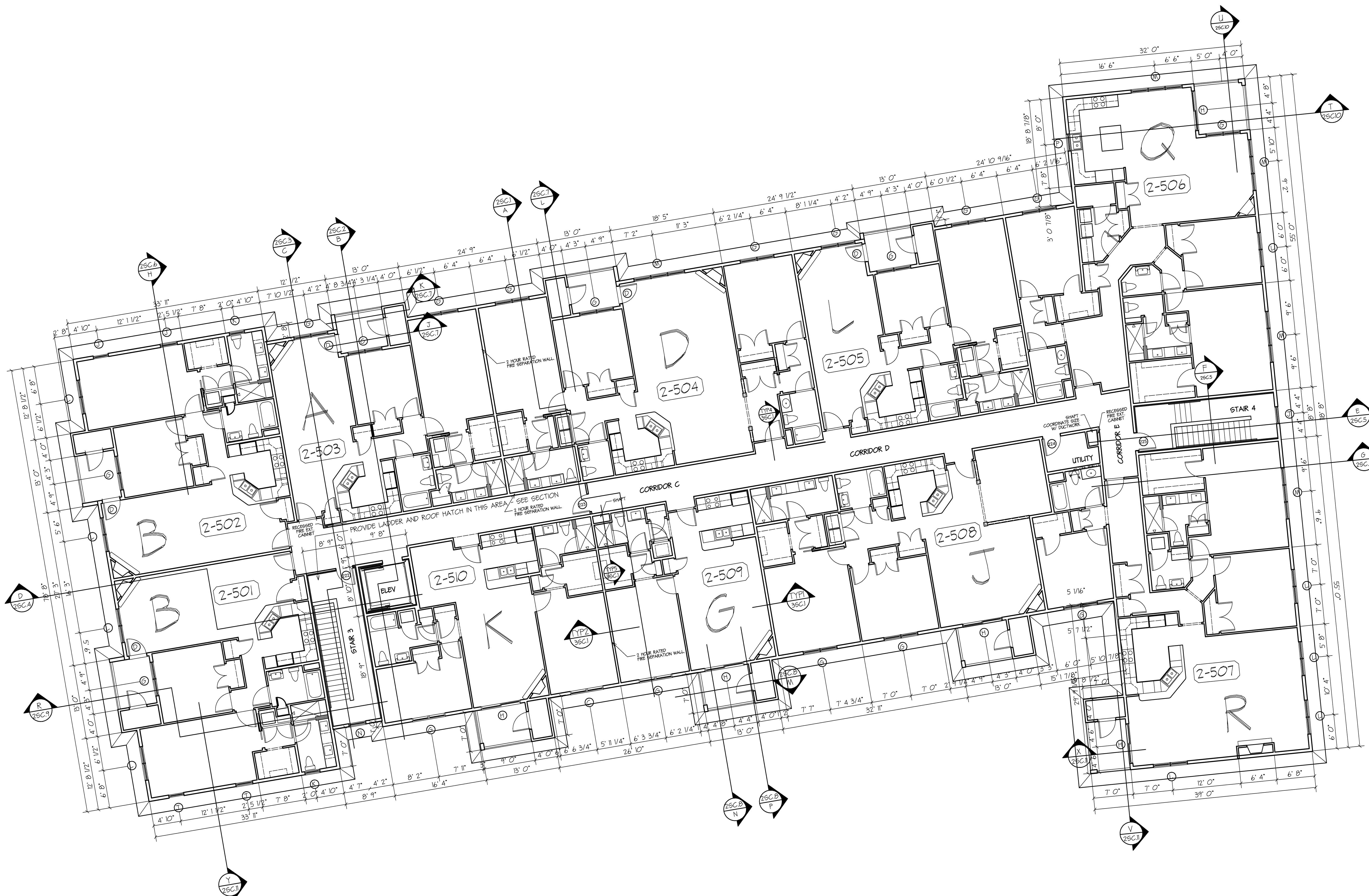
5th FLOOR PLAN PHASE I, BUILDING 2 SCALE: 1/8" = 1' 0" GROSS FLOOR AREA INCLUDING DECKS: 16,817 SF
