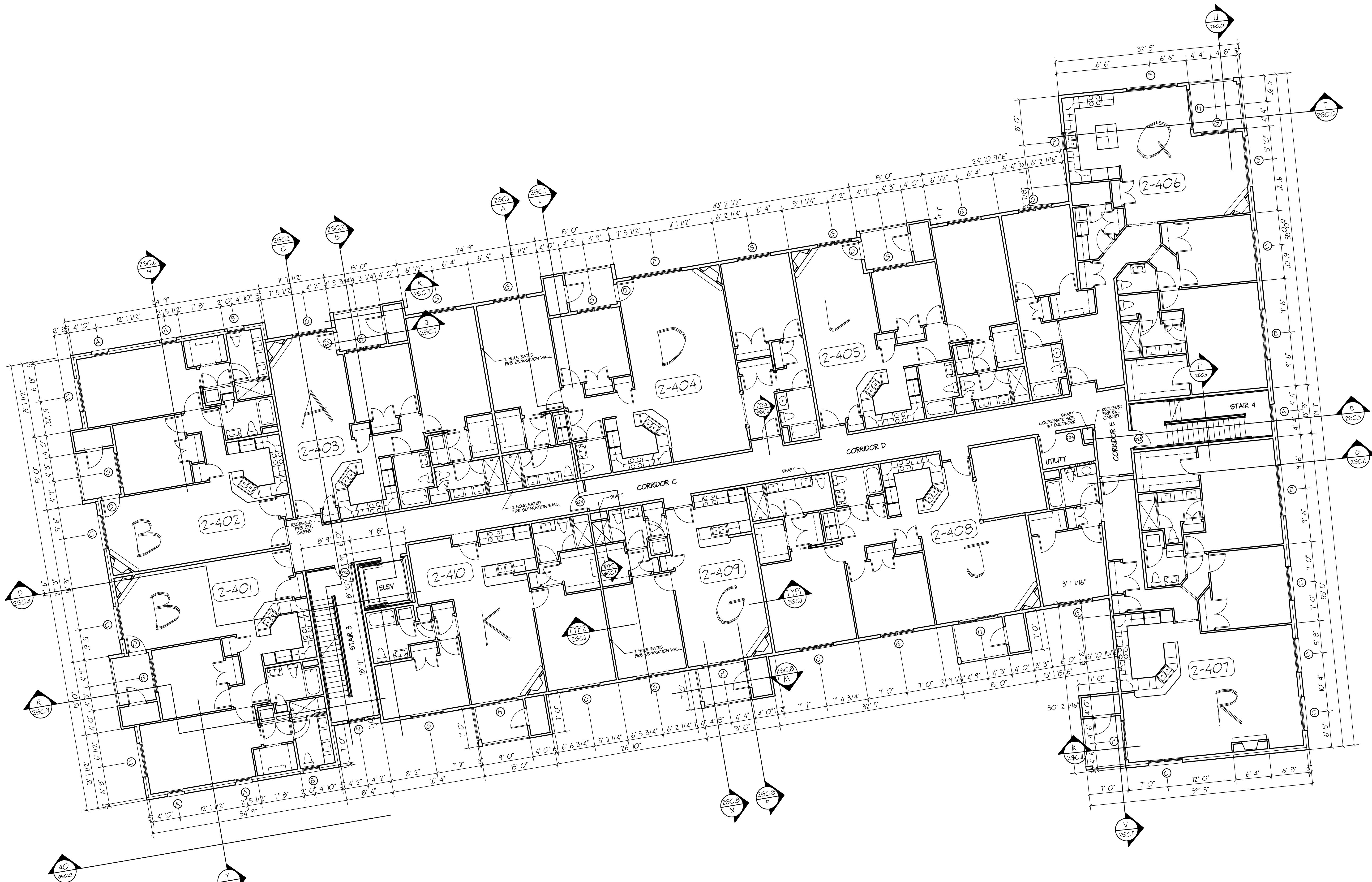
4th FLOOR PLAN PHASE I, BUILDING 2 SCALE: 1/8" = 1' 0" GROSS FLOOR AREA INCLUDING DECKS: 16,991 SF
