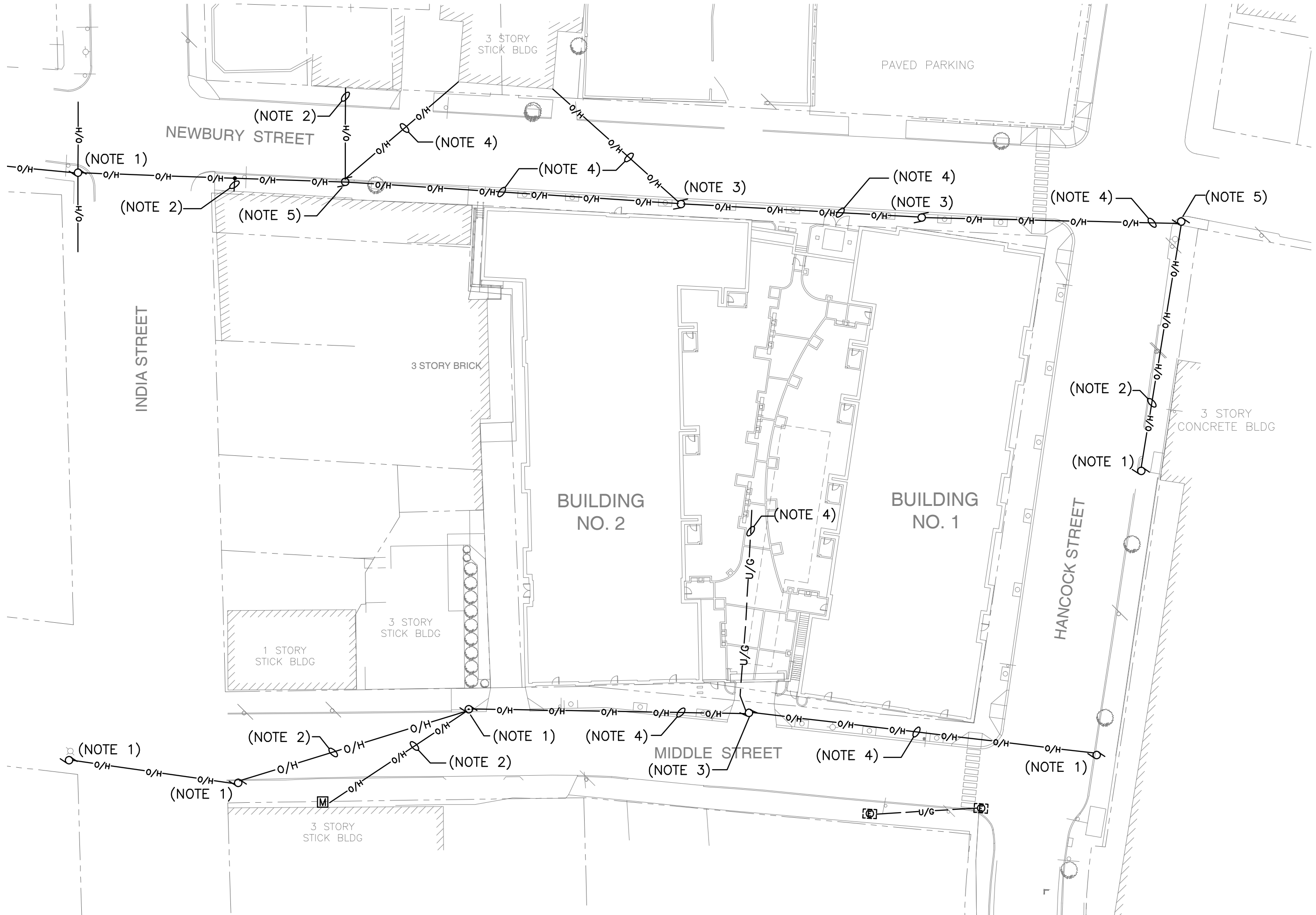
ELECTRICAL REMOVALS PLAN 1" = 40'-0"
