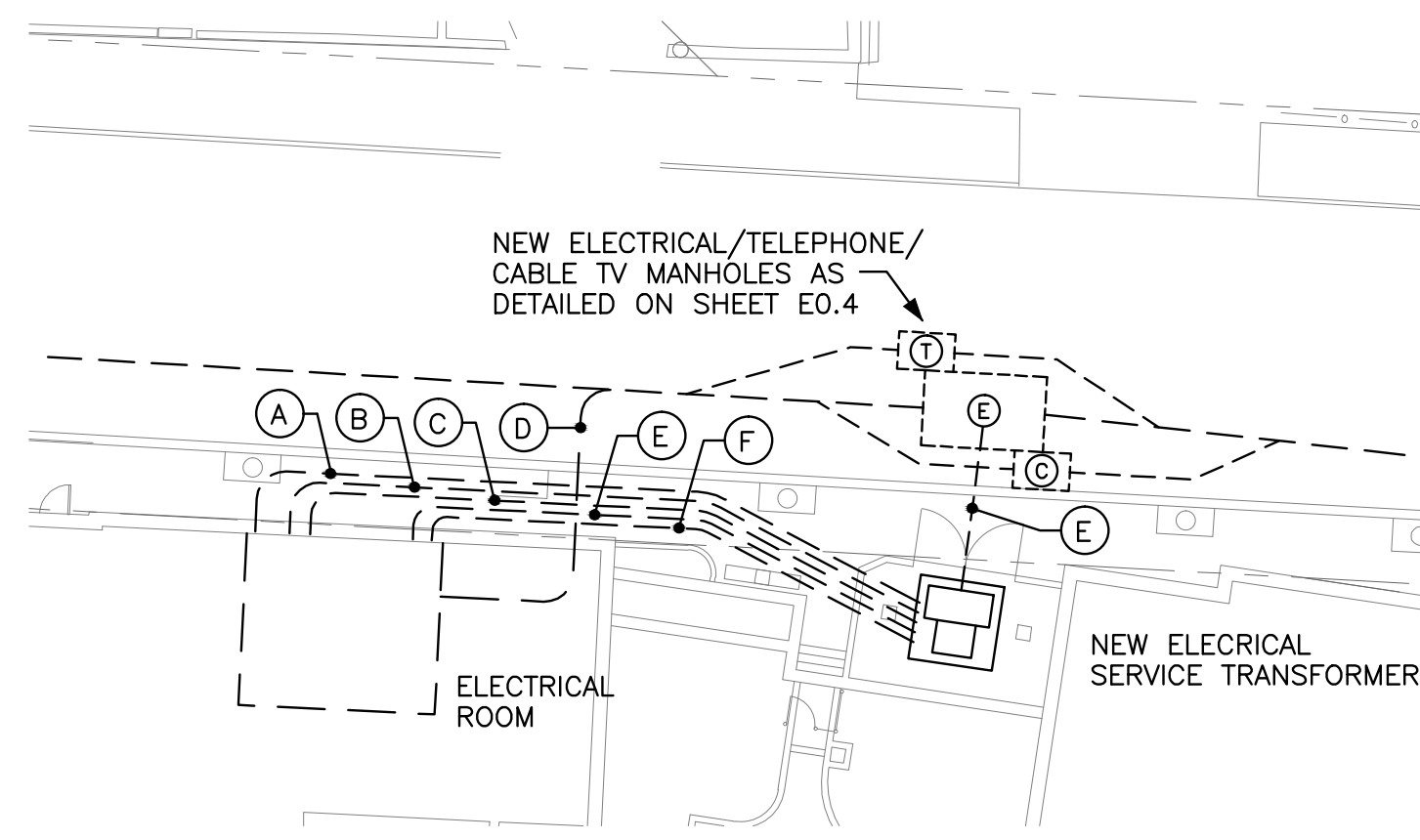
ELECTRICAL SERVICE ENTRANCE DETAIL PLAN 1" = 10'-0"
