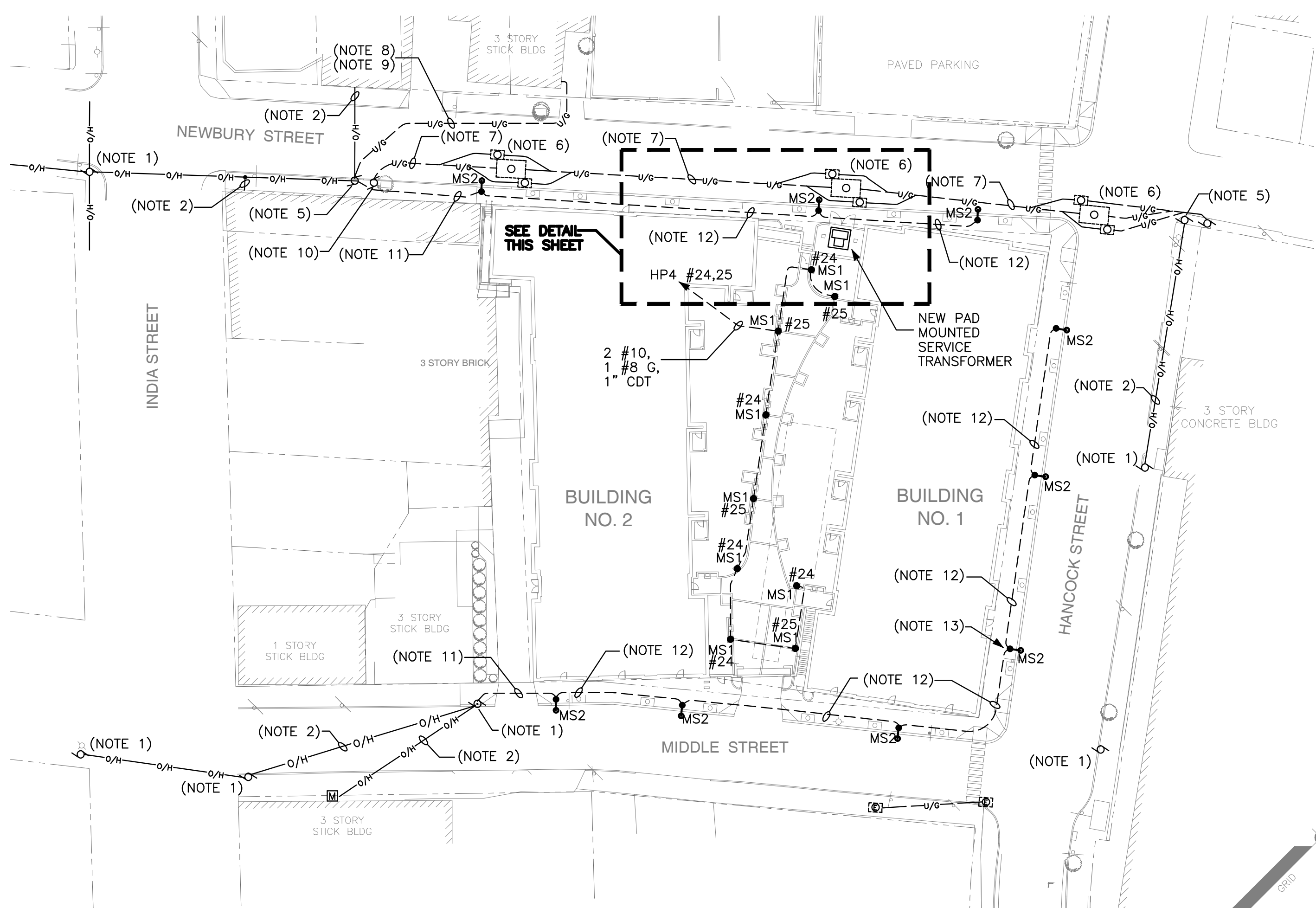
PROPOSED ELECTRICAL SITE PLAN 1" = 40'-0"
