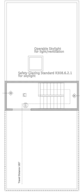
30 FOURTH FLOOR PLAN SCALE: 1/8" = 1'-0"
