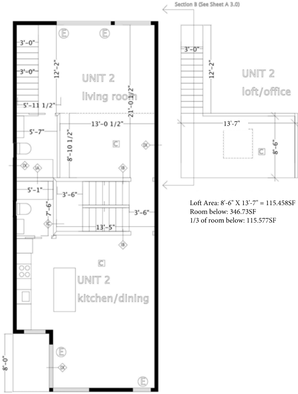
30 THIRD FLOOR PLAN SCALE: 1/8" = 1'-0"
