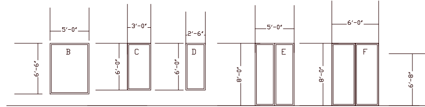
WINDOW AND DOOR SCHEDULE
