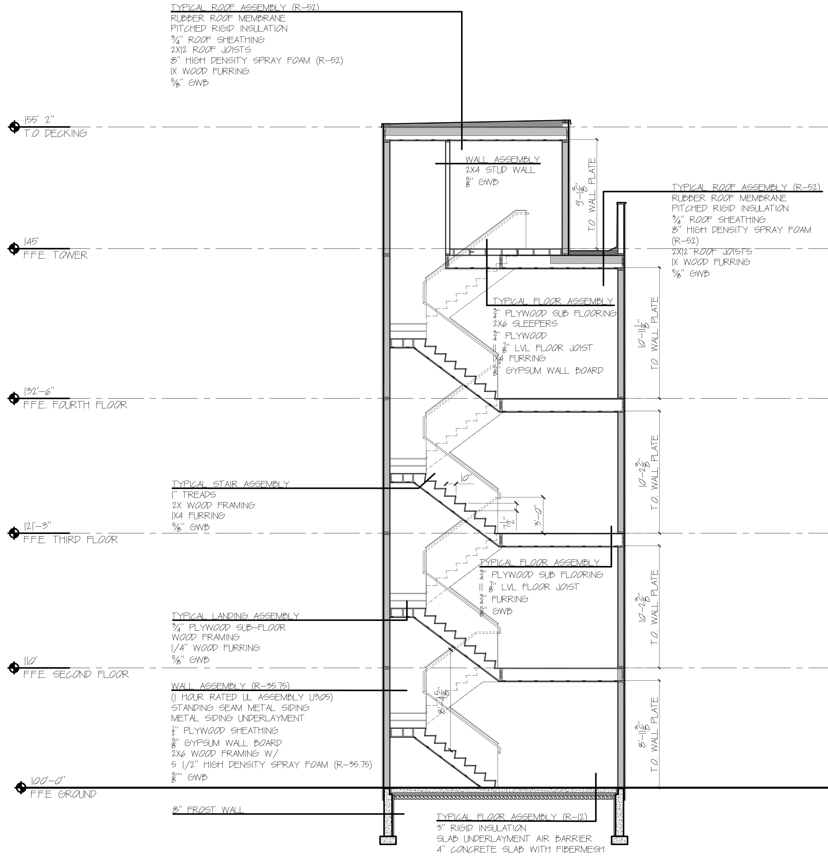
10 BUILDING SECTION 0 4'-0" SCALE: 1/4" = 1'-0"
