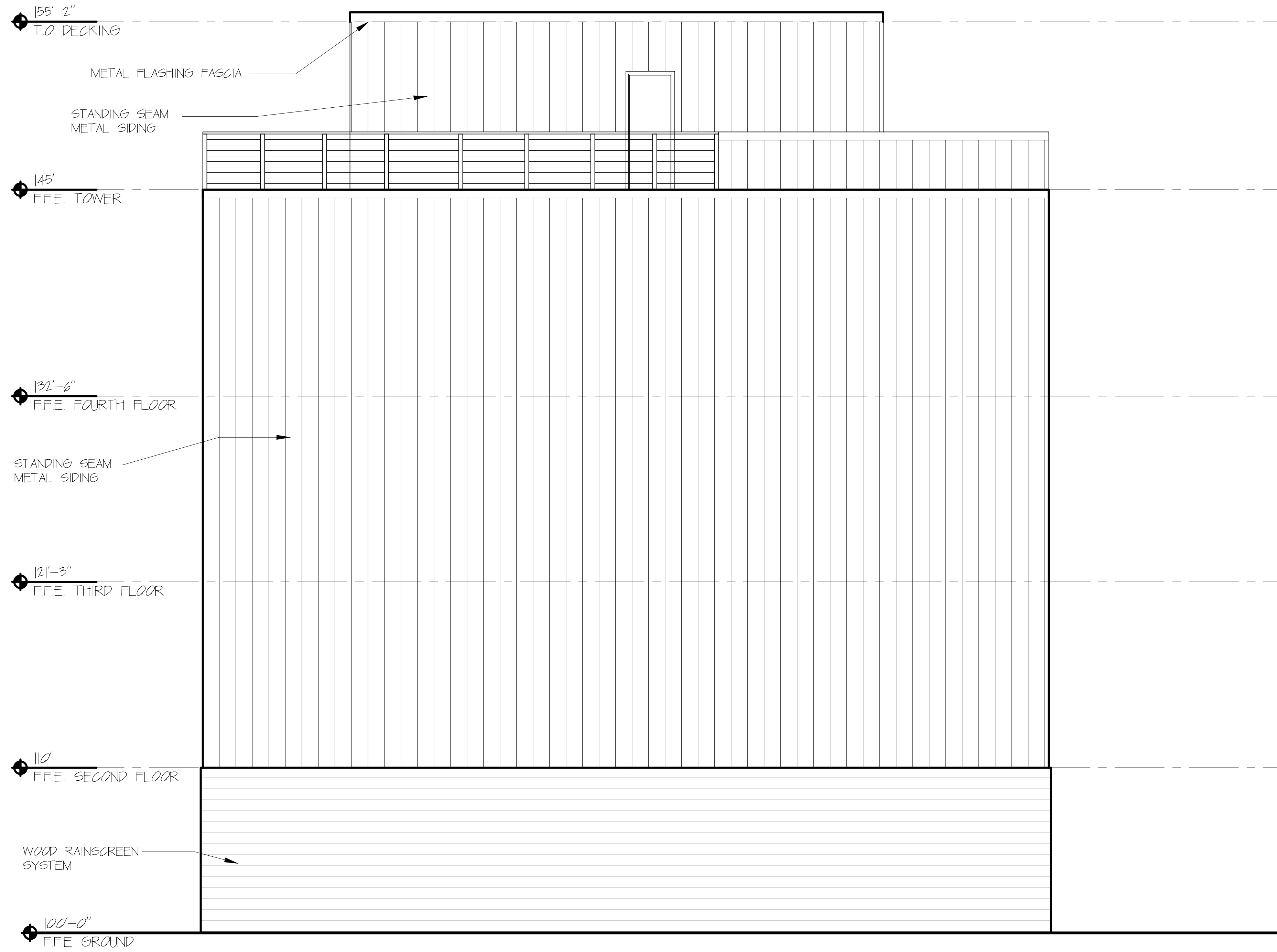
10 NORTH ELEVATION 1/1/15 0 4'-0" SCALE: 1/4" = 1'-0"
