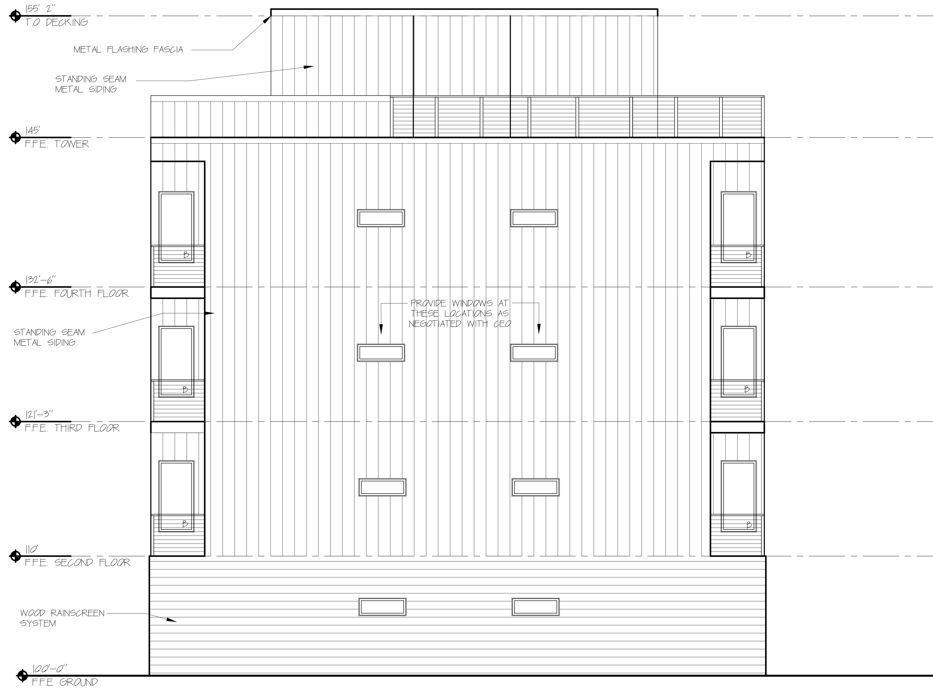
10 SOUTH ELEVATION 1/4" = 1'-0"
