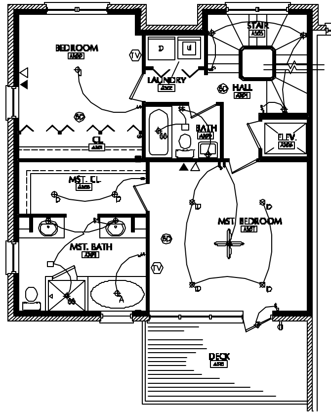
3 ELECT. PLAN - 3rd FLOOR SCALE: 1/4" = 1'-0"
