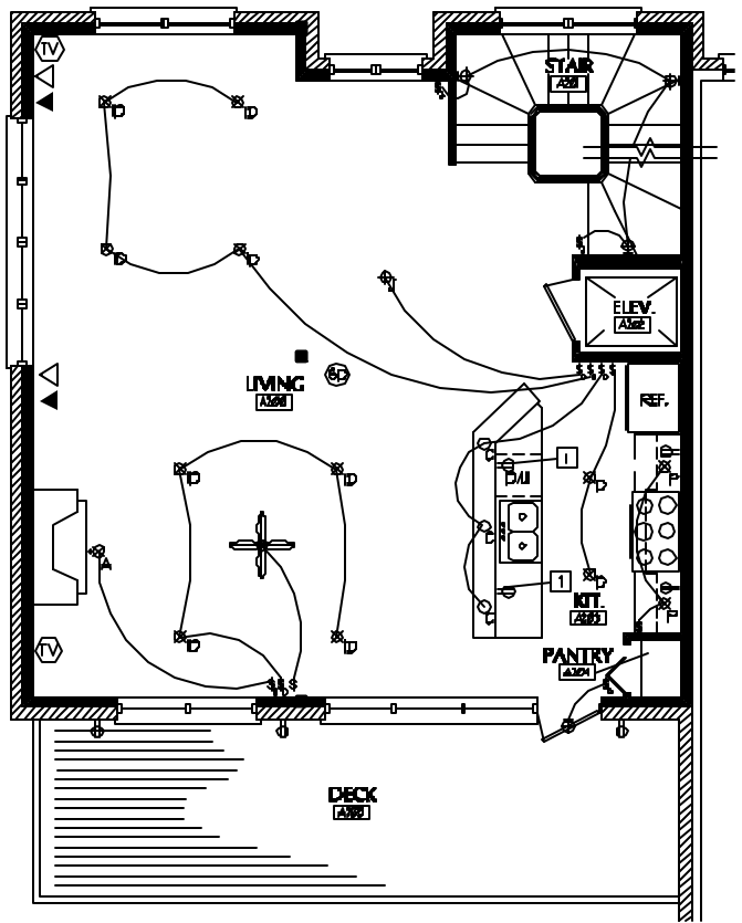
2 ELECT. PLAN - 2nd FLOOR SCALE: 1/4" = 1'-0"
