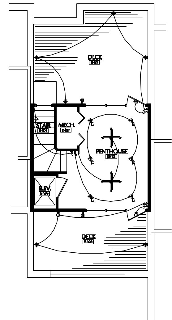
4 ELECT. PLAN - 4th FLOOR SCALE: 1/4" = 1'-0"
