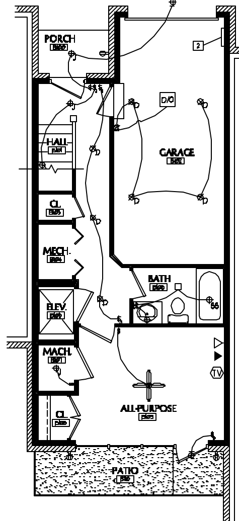
1 ELECT. PLAN - 1st FLOOR SCALE: 1/4" = 1'-0"
