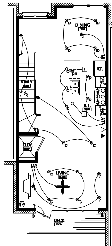
2 ELECT. PLAN - 2nd FLOOR SCALE: 1/4" = 1'-0"
