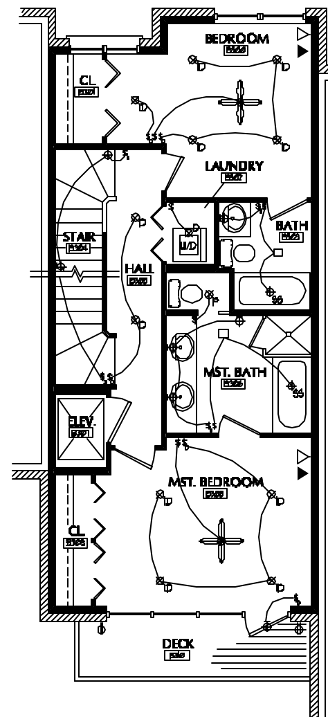
3 ELECT. PLAN - 3rd FLOOR SCALE: 1/4" = 1'-0"
