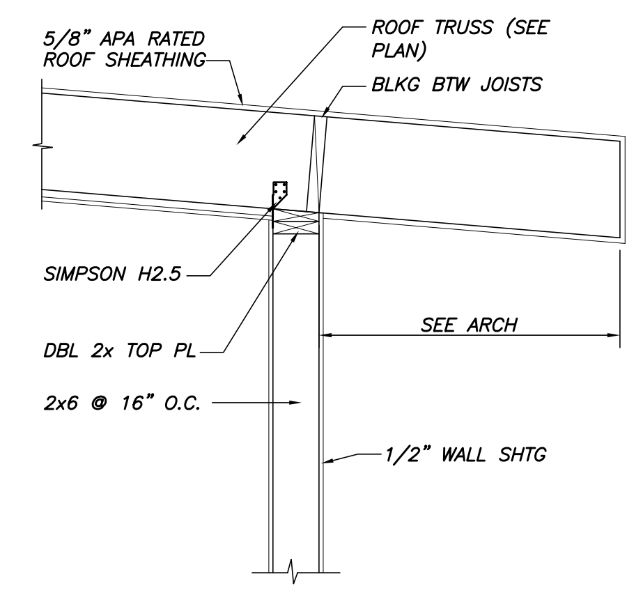
SECTION 3 3/4"=1'-0" S1.5
