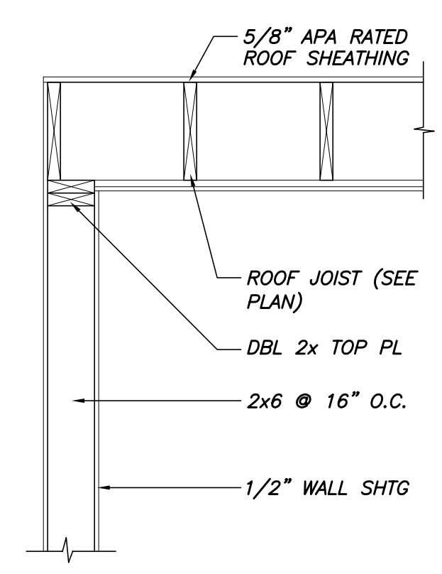
SECTION 2 3/4"=1'-0" S1.5
