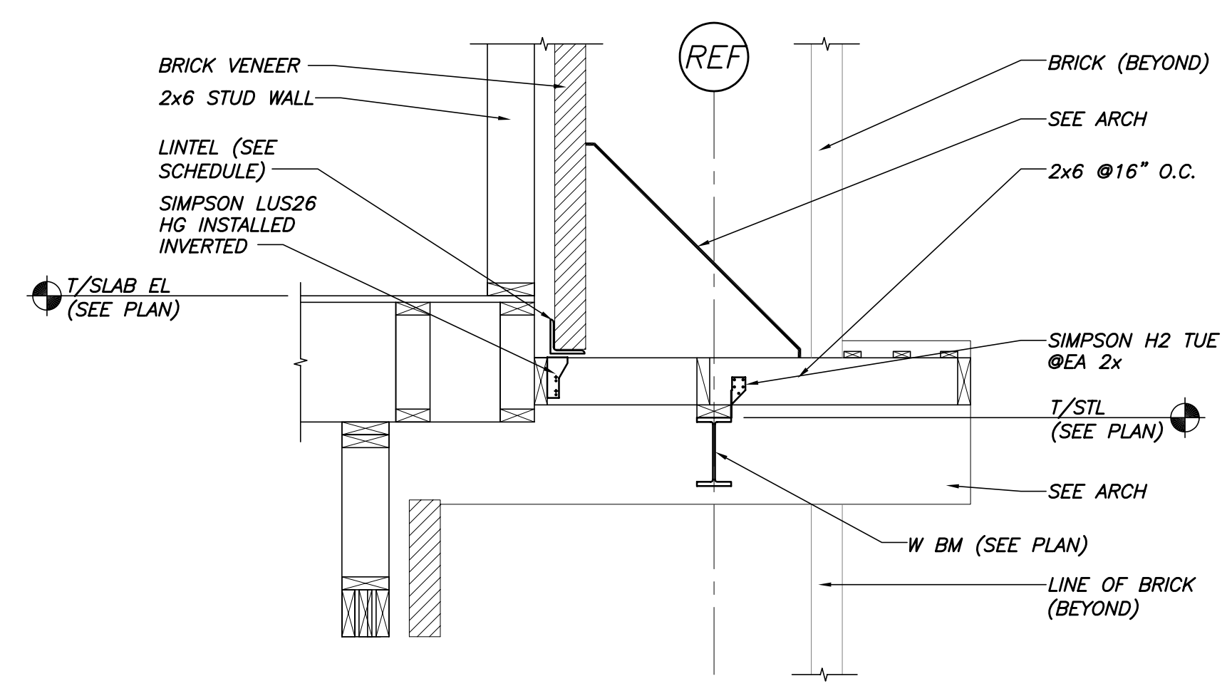
SECTION 9 3/4"=1'-0" S1.2
