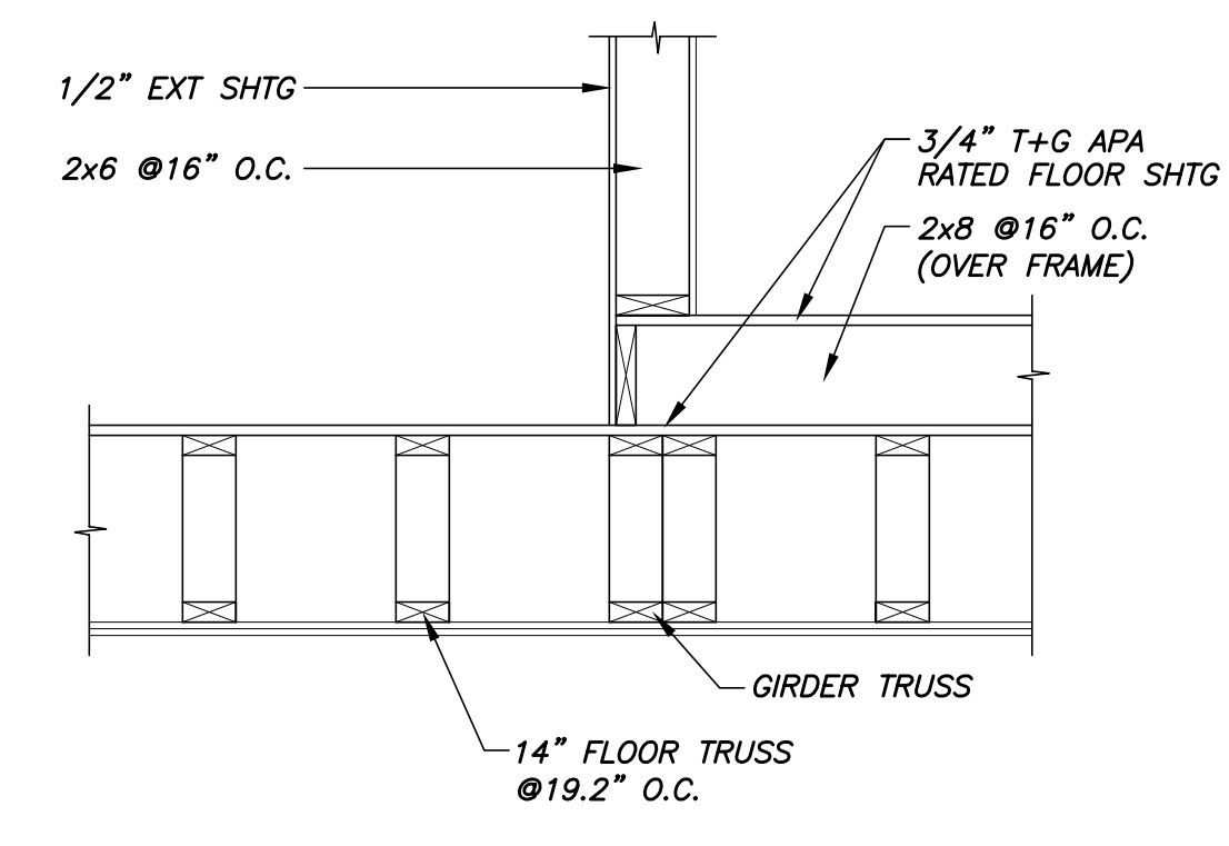
SECTION 5 3/4"=1'-0" S1.4
