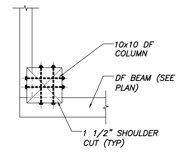
SECTION 8 3/4"=1'-0" S1.4
