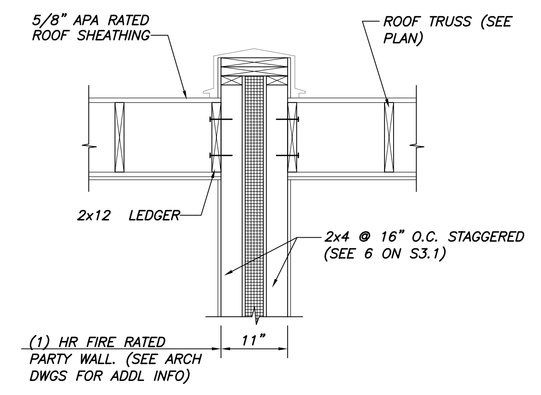
SECTION 4 3/4"=1'-0" S1.5
