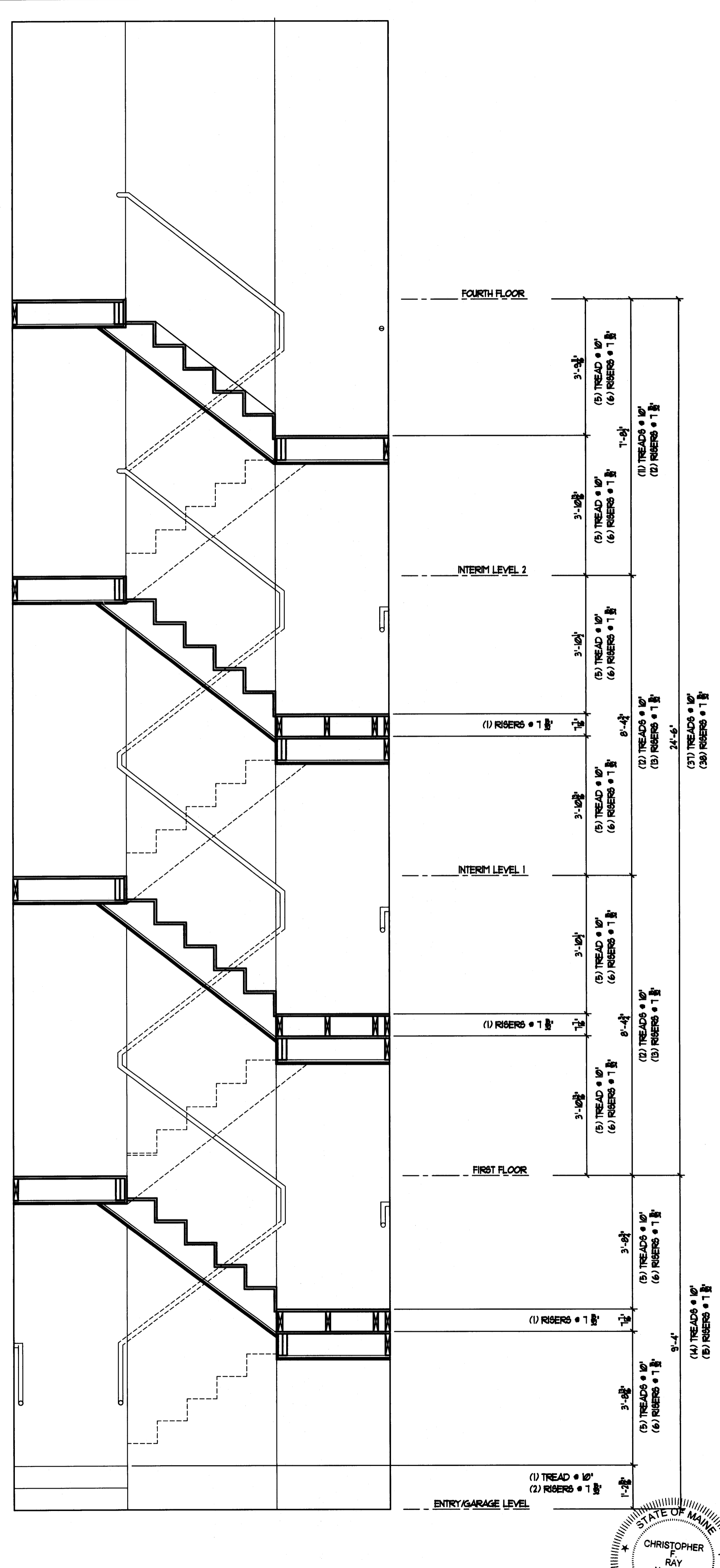
SECTION THROUGH SECONDARY STAIR SCALE: 1/2" = 1'-0"
