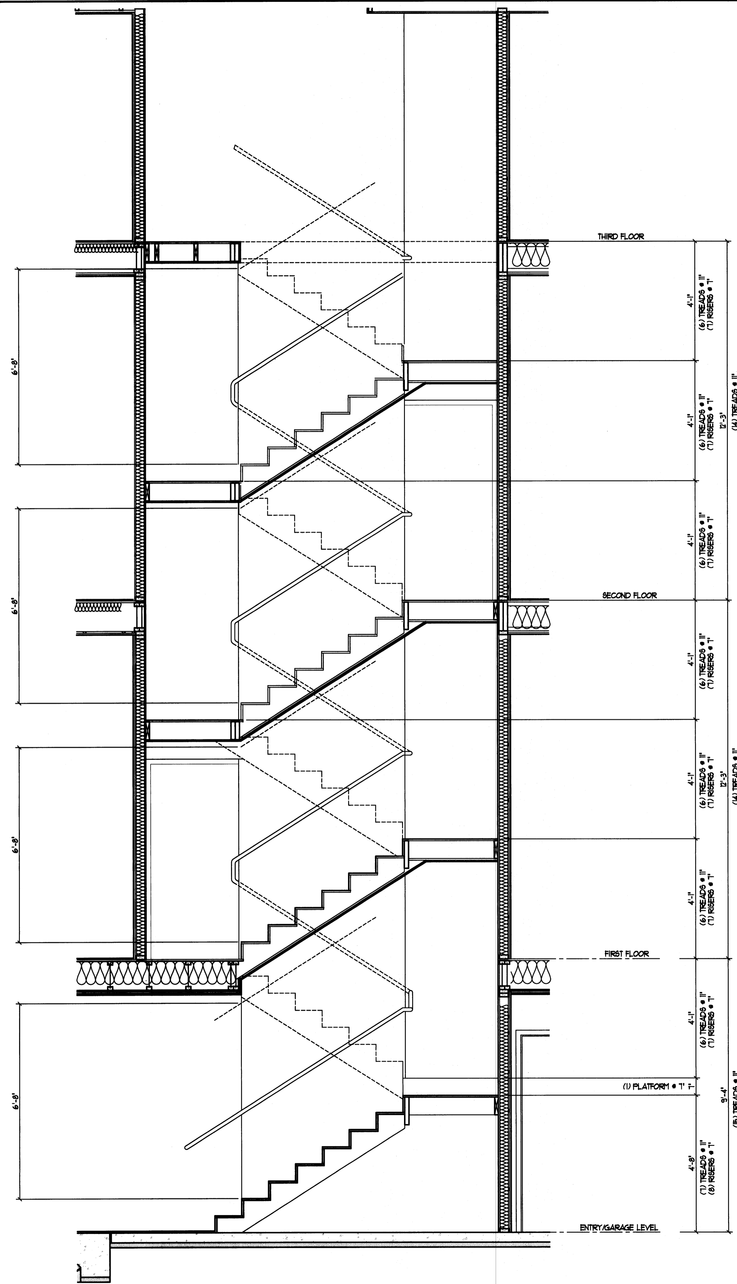
SECTION THROUGH MAIN STAIR SCALE: 1/2" = 1'-0"
